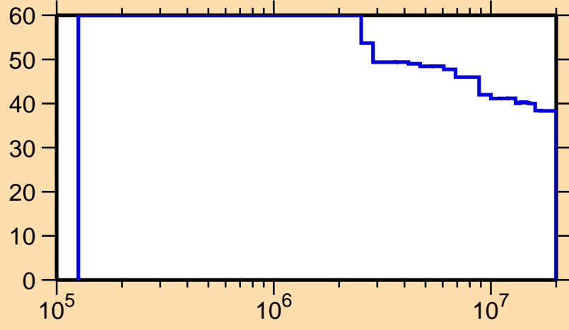
\Delta\sigma/\sigma vs. E for ^{81}\text{Zr}(n,n_1)
