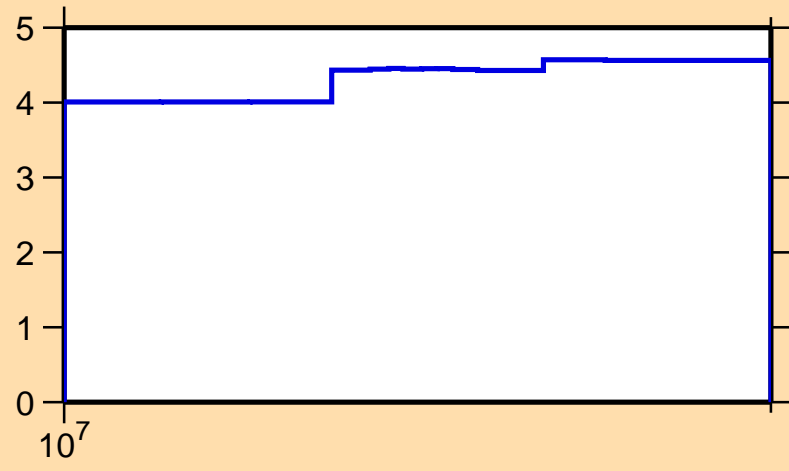
\Delta\sigma/\sigma vs. E for ^{81}\text{Zr}(n,\text{nonel.})
