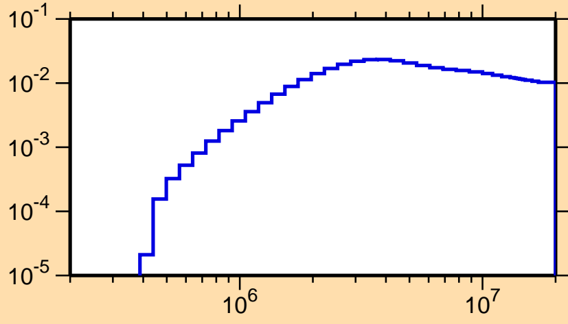
\sigma vs. E for ^{81}\text{Zr}(n,n\text{cont.})
