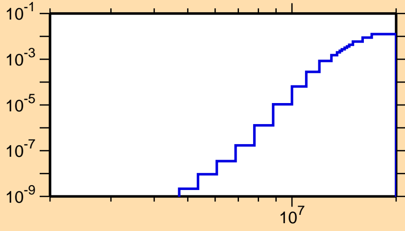
\sigma vs. E for ^{81}\text{Zr}(n,\text{He3})
