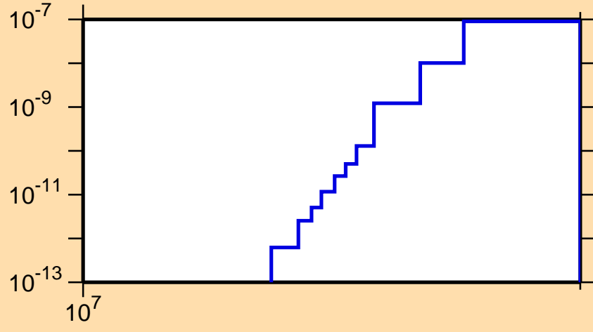
\sigma vs. E for ^{81}\text{Zr}(\text{mt117})
