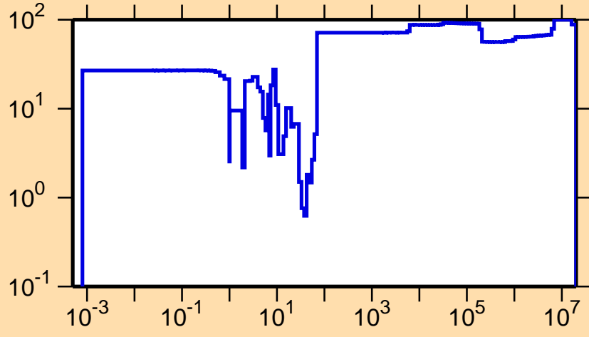
\Delta\sigma/\sigma vs. E for ^{81}\text{Zr}(n,\gamma)
