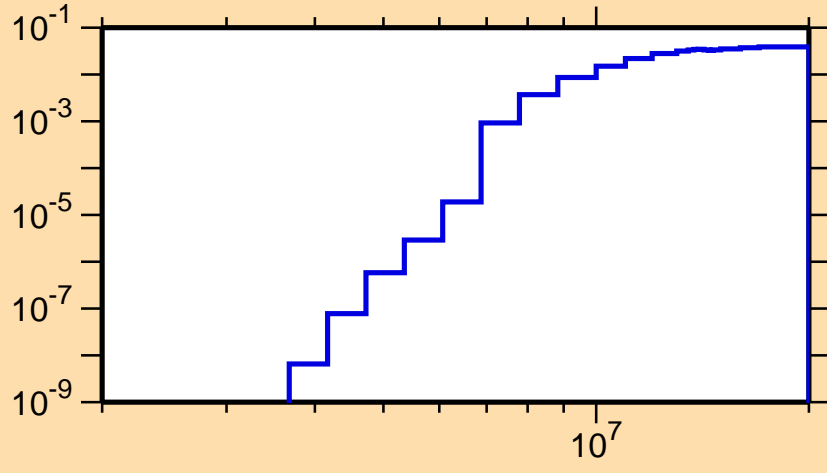
\sigma vs. E for ^{81}\text{Zr}(n,d)
