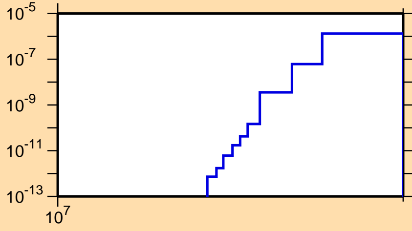
\sigma vs. E for ^{81}\text{Zr} (mt 45)
