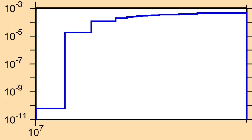
\sigma vs. E for ^{81}\text{Zr}(n,2n)
