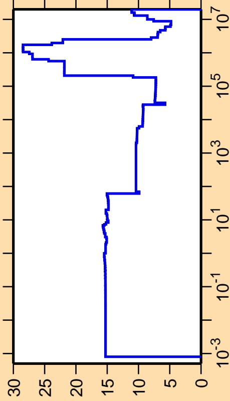
\Delta\sigma/\sigma vs. E for ^{81}\text{Zr}(n,\text{el.})
