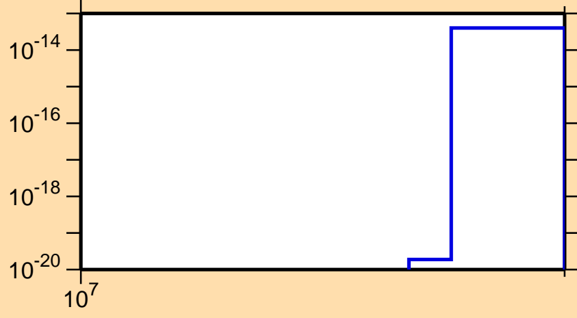
\sigma vs. E for ^{81}\text{Zr}(n,2n\alpha)
