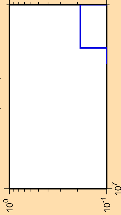
\Delta\sigma/\sigma vs. E for ^{81}\text{Zr}(n,2n\alpha)
