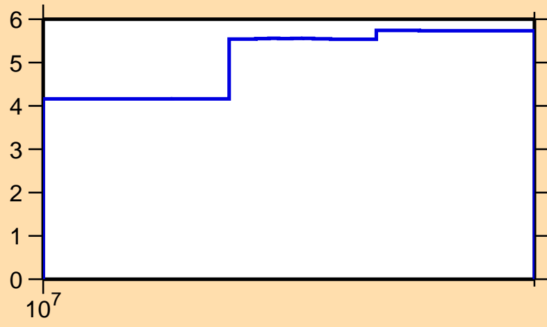
\Delta\sigma/\sigma vs. E for ^{81}\text{Zr}(n,\text{tot.})
