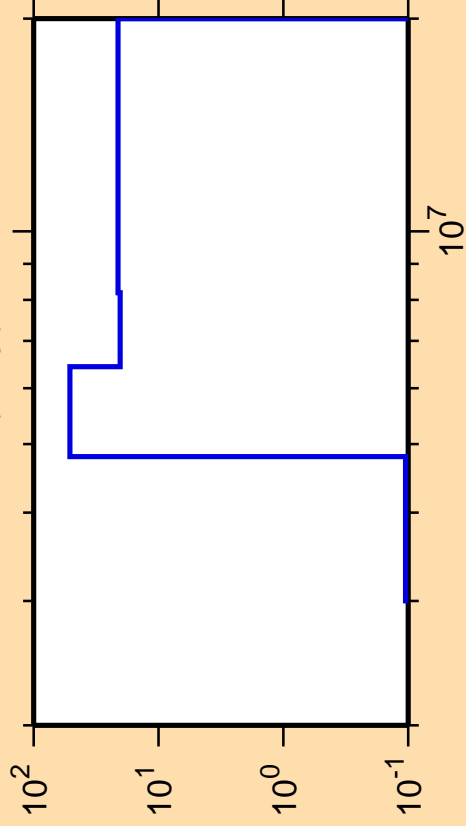
\Delta\sigma/\sigma vs. E for ^{81}\text{Zr}(n,np)
