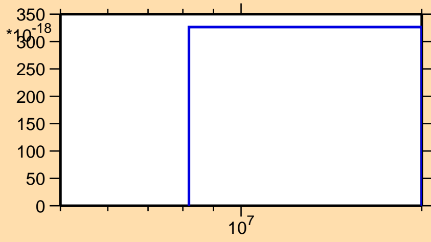
\sigma vs. E for ^{81}\text{Zr}(n,2n\alpha)
