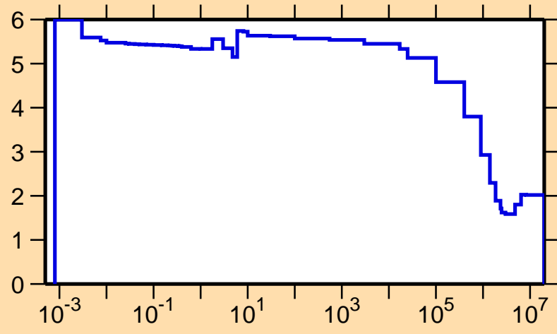
\sigma vs. E for ^{81}\text{Zr}(n,\text{el.})
