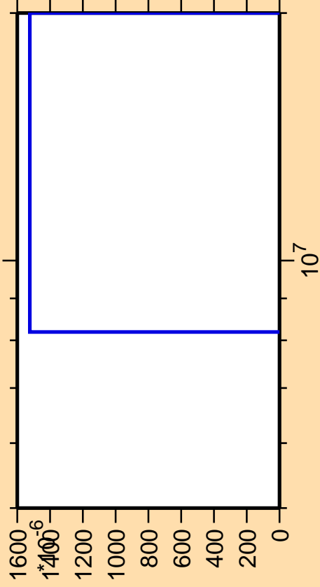
\Delta\sigma/\sigma vs. E for ^{81}\text{Zr}(n,2n\alpha)
