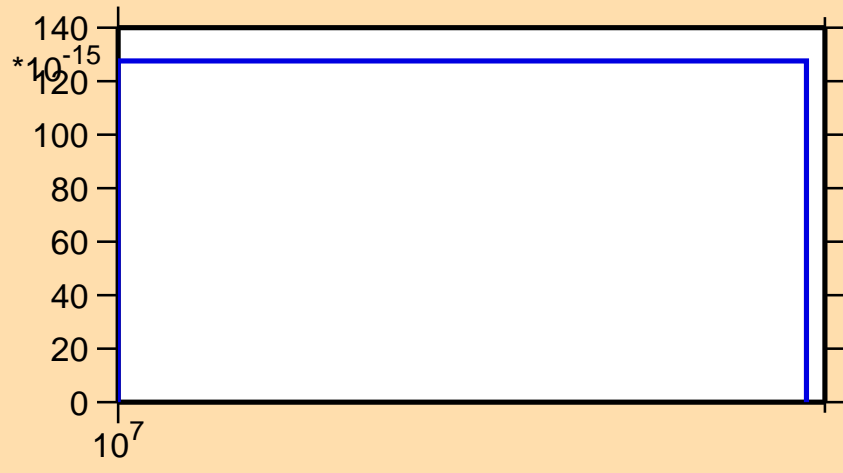
\sigma vs. E for ^{82}\text{Zr} (mt 34)
