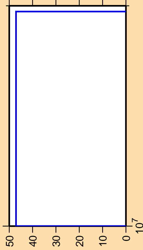
\Delta\sigma/\sigma vs. E for ^{82}\text{Zr} (mt 45)
