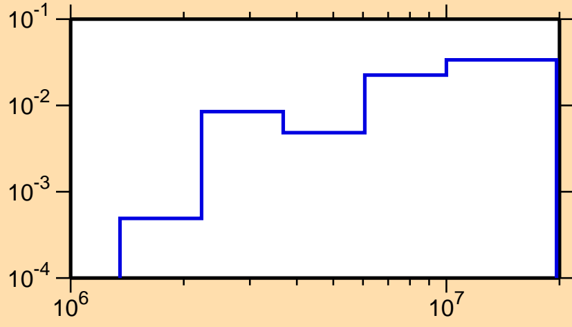
\sigma vs. E for ^{82}\text{Zr}(n,n\text{cont.})
