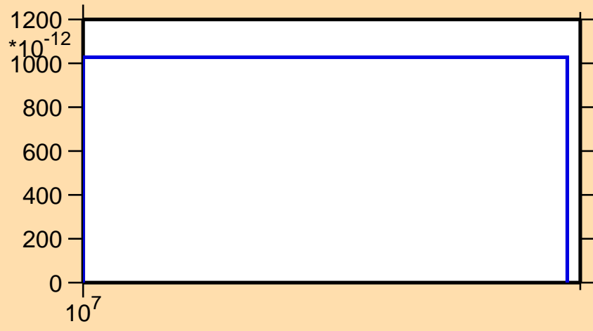
\sigma vs. E for ^{82}\text{Zr} (mt 45)
