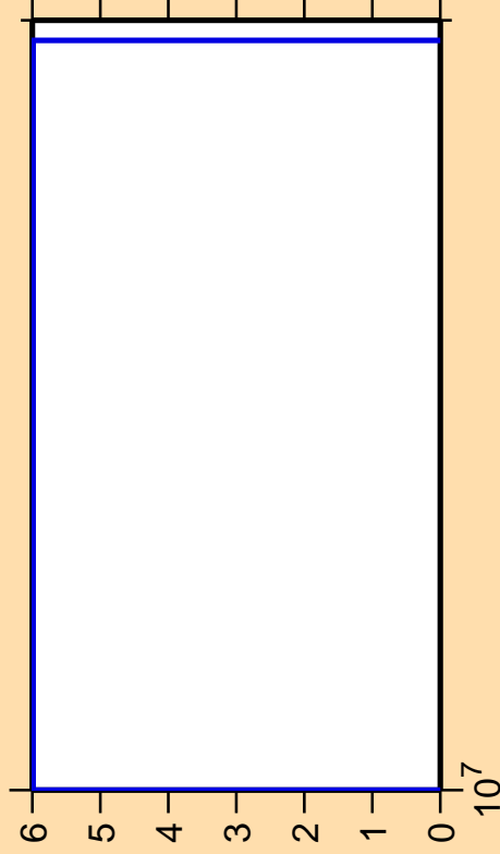
\Delta\sigma/\sigma vs. E for ^{82}\text{Zr}(n,2np)
