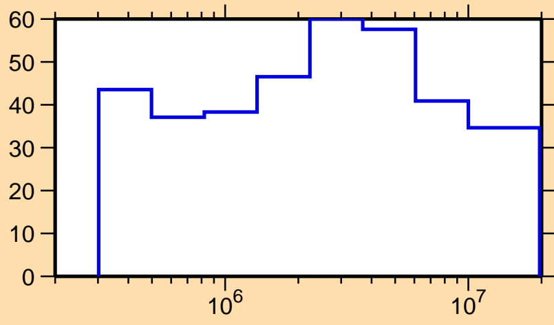
\Delta\sigma/\sigma vs. E for ^{82}\text{Zr}(n,n_1)
