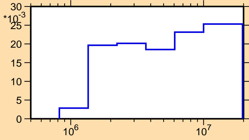
\sigma vs. E for ^{82}\text{Zr}(n,n_3)
