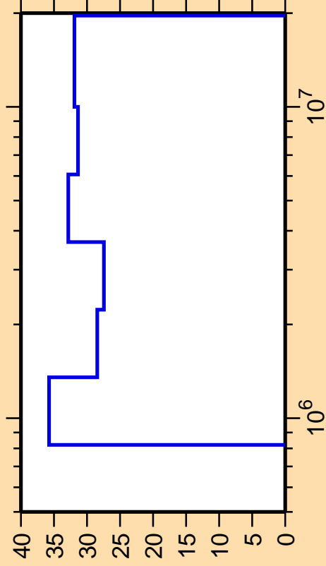
\Delta\sigma/\sigma vs. E for ^{82}\text{Zr}(n,n_3)
