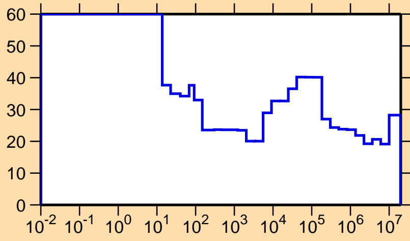
\Delta\sigma/\sigma vs. E for ^{82}\text{Zr}(n,p)
