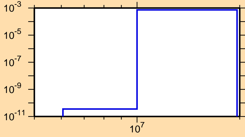
\sigma vs. E for ^{82}\text{Zr}(n,\text{pd})
