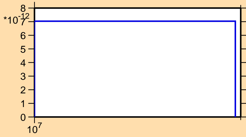
\sigma vs. E for ^{82}\text{Zr}(n,nd)
