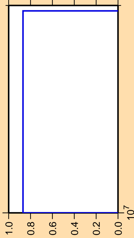
\Delta\sigma/\sigma vs. E for ^{82}\text{Zr} (mt 34)
