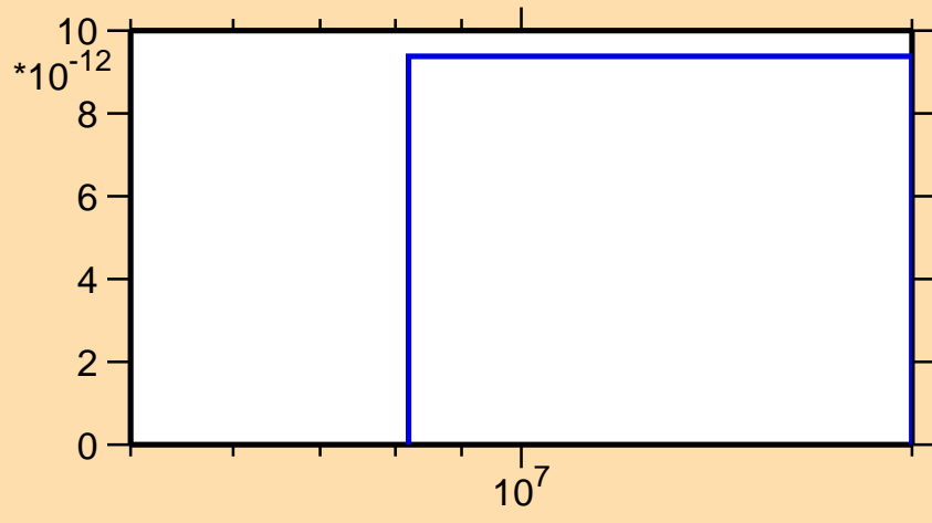
\sigma vs. E for ^{82}\text{Zr}(n,nd)
