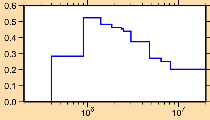
\sigma vs. E for ^{82}\text{Zr}(n,\text{inel.})
