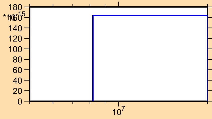
\sigma vs. E for ^{82}\text{Zr}(\text{mt } 34)
