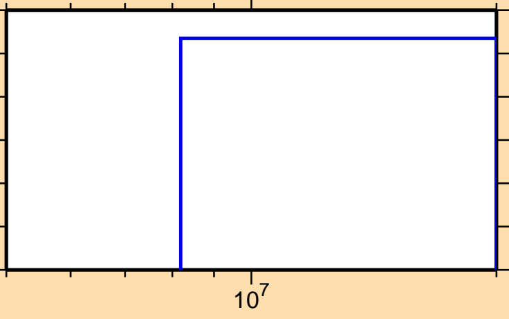
\sigma vs. E for ^{82}\text{Zr}(n,\text{pt})
