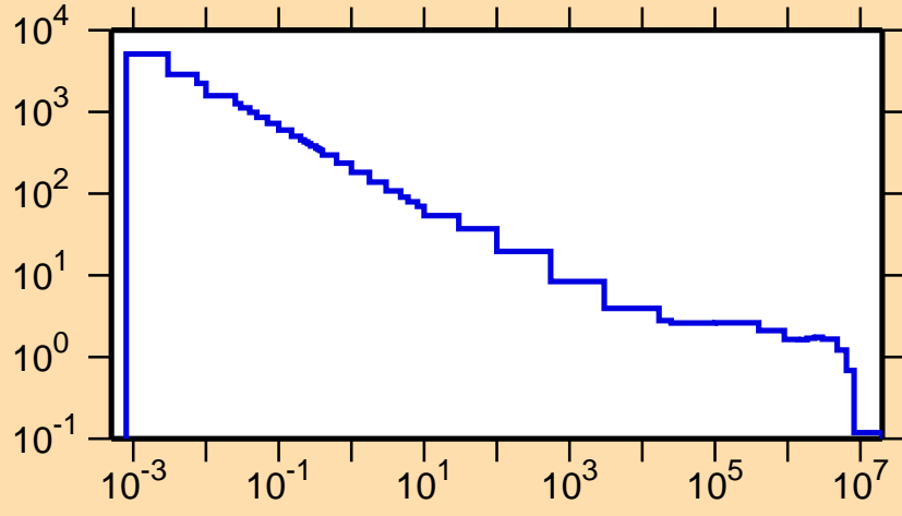
\sigma vs. E for ^{82}\text{Zr}(n,p)
