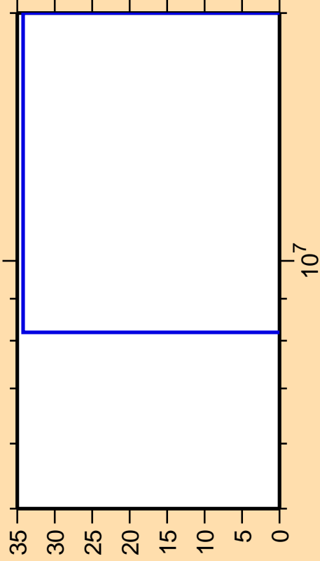
\Delta\sigma/\sigma vs. E for ^{82}\text{Zr}(n,nd)
