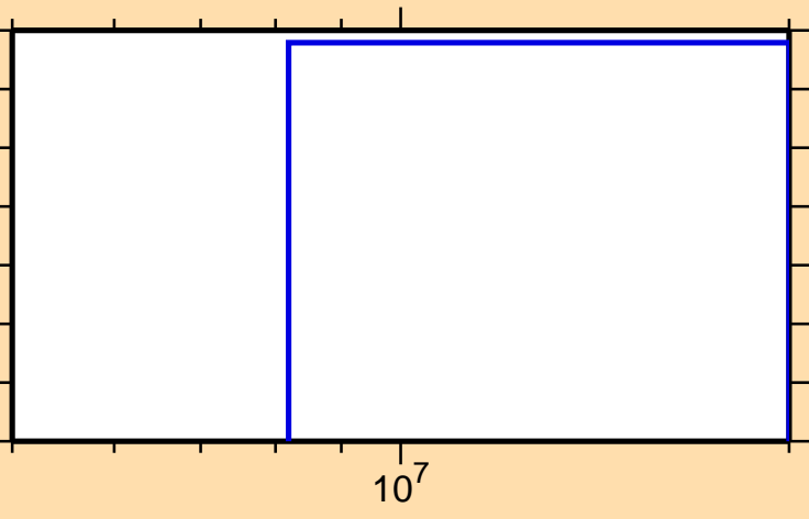
\sigma vs. E for ^{82}\text{Zr}(n,2n)
