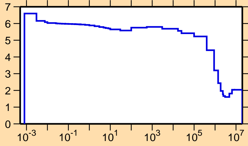
\sigma vs. E for ^{82}\text{Zr}(n,\text{el.})
