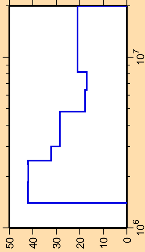
\Delta\sigma/\sigma vs. E for ^{82}\text{Zr}(n,n_4)
