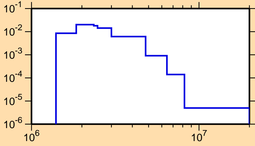
\sigma vs. E for ^{82}\text{Zr}(n,n_4)
