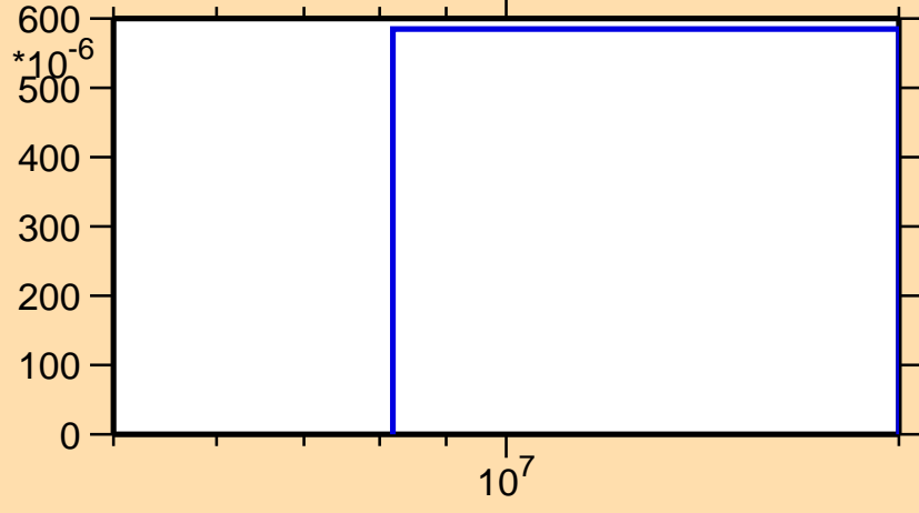
\sigma vs. E for ^{82}\text{Zr}(n,\text{pd})
