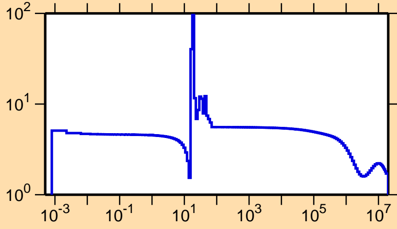
\sigma vs. E for ^{83}\text{Zr}(n,\text{el.})
