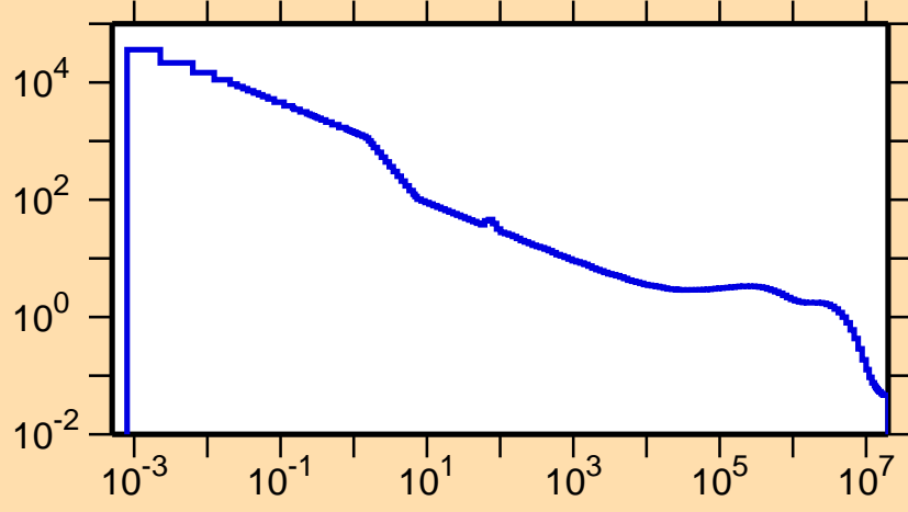
\sigma vs. E for ^{83}\text{Zr}(n,p)
