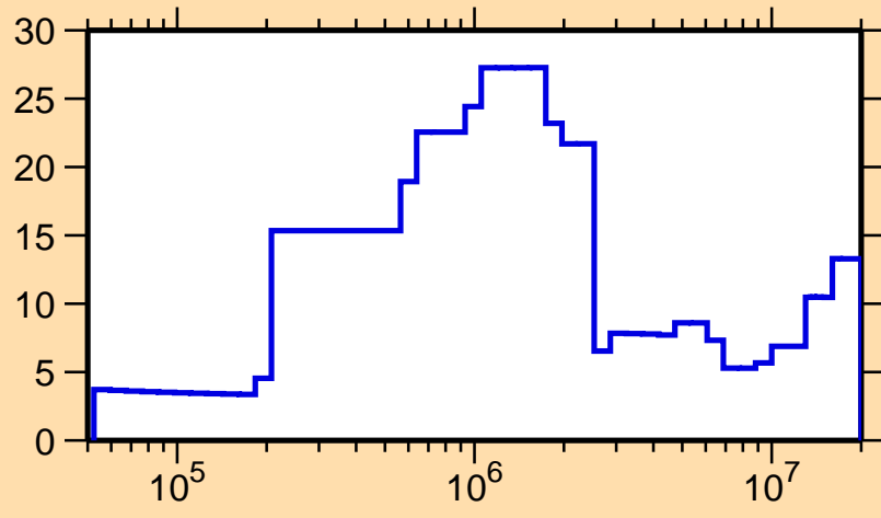
\Delta\sigma/\sigma vs. E for ^{83}\text{Zr}(n,\text{el.})
