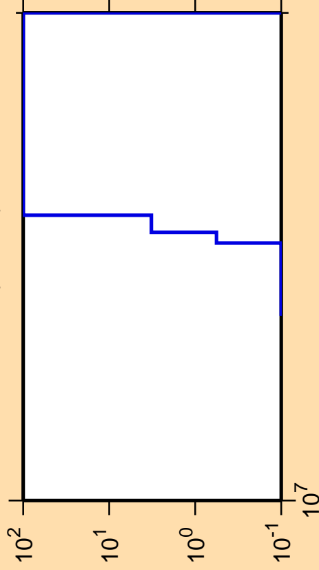
\Delta\sigma/\sigma vs. E for ^{83}\text{Zr} (mt 34)
