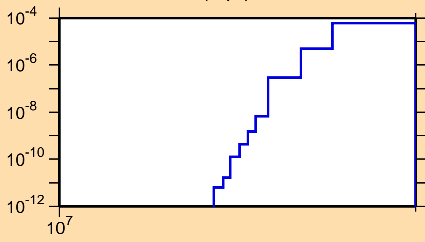
\sigma vs. E for ^{83}\text{Zr}(n,\text{pt})
