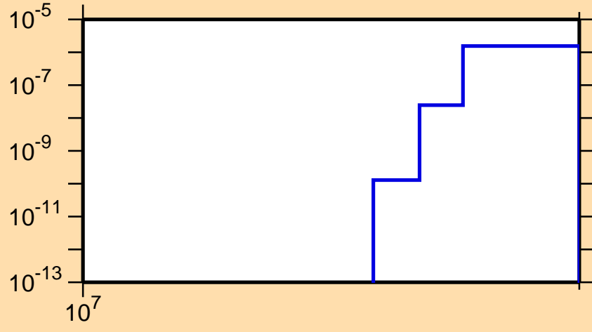
\sigma vs. E for ^{83}\text{Zr}(n,\text{nd})
