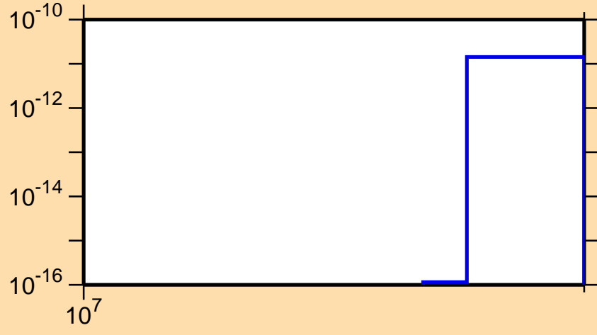
\sigma vs. E for ^{83}\text{Zr}(n,2n\alpha)
