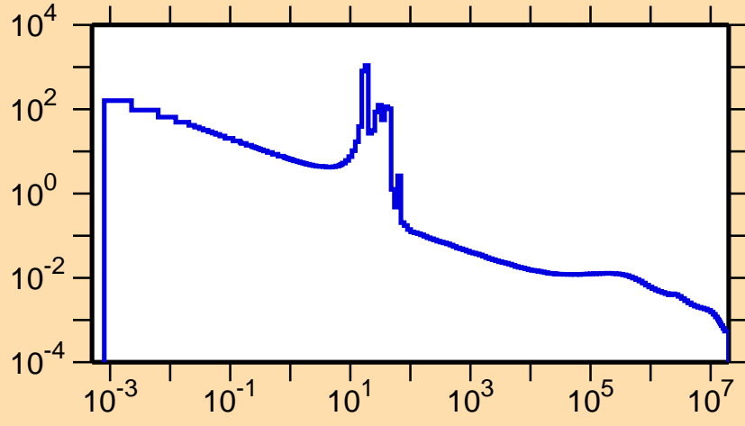
\sigma vs. E for ^{83}\text{Zr}(n,\gamma)
