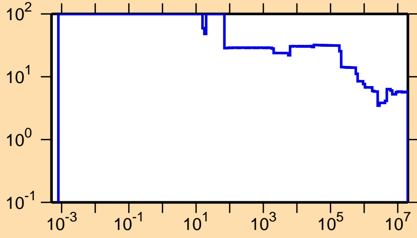
\Delta\sigma/\sigma vs. E for ^{83}\text{Zr}(n,\text{nonel.})
