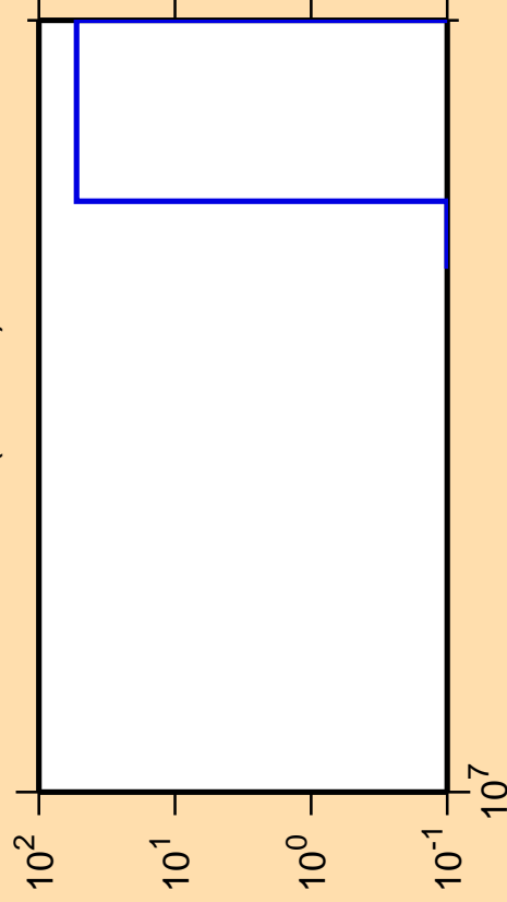
\Delta\sigma/\sigma vs. E for ^{83}\text{Zr}(n,2n\alpha)
