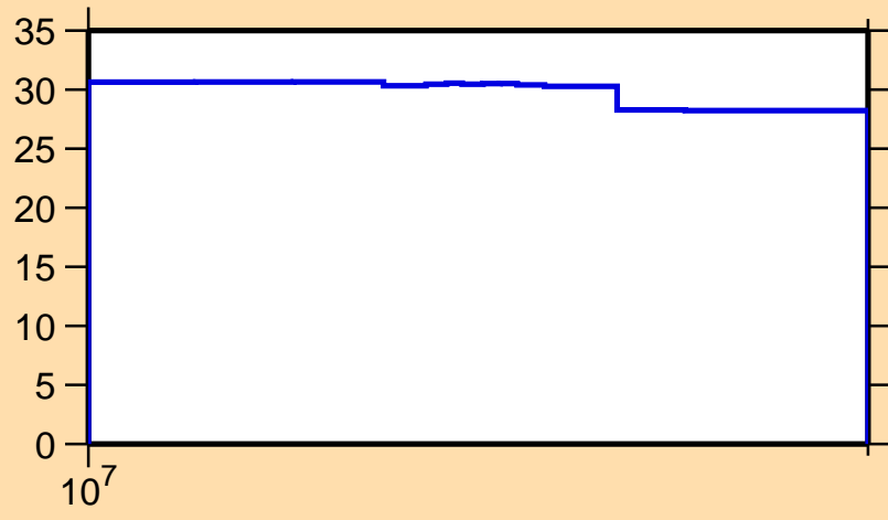
\Delta\sigma/\sigma vs. E for ^{83}\text{Zr}(n,\text{inel.})
