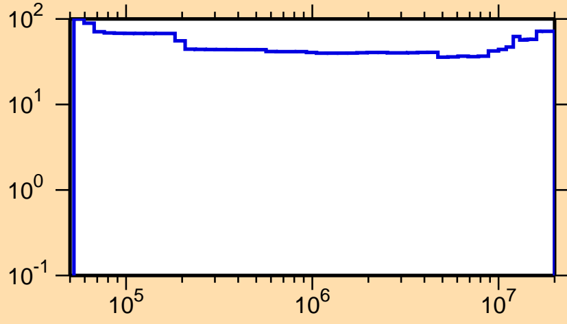
\Delta\sigma/\sigma vs. E for ^{83}\text{Zr}(n,n_1)
