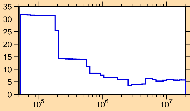
\Delta\sigma/\sigma vs. E for ^{83}\text{Zr}(n,\text{nonel.})
