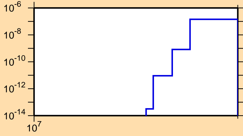
\sigma vs. E for ^{83}\text{Zr} (mt 45)
