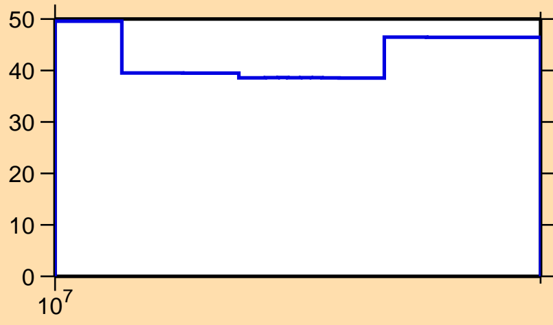
\Delta\sigma/\sigma vs. E for ^{83}\text{Zr}(n,2n)
