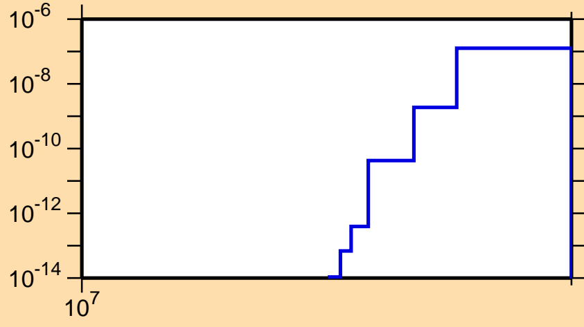
\sigma vs. E for ^{83}\text{Zr} (mt 34)
