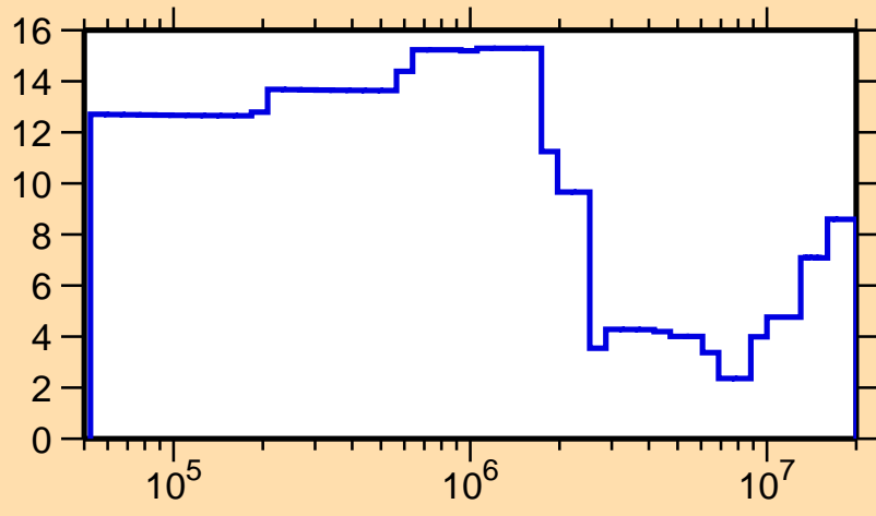
\Delta\sigma/\sigma vs. E for ^{83}\text{Zr}(n,\text{tot.})
