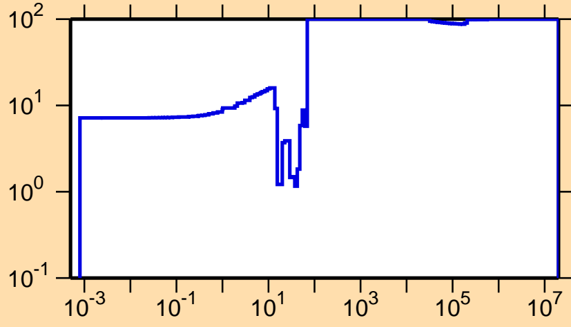
\Delta\sigma/\sigma vs. E for ^{83}\text{Zr}(n,\gamma)
