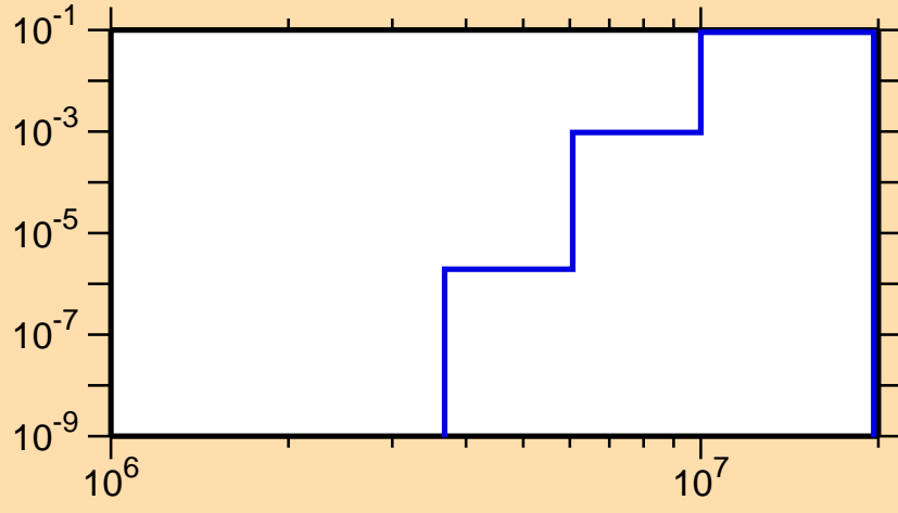
\sigma vs. E for ^{83}\text{Zr}(n,p\alpha)
