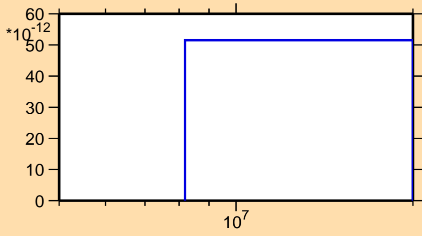
\sigma vs. E for ^{83}\text{Zr}(\text{mt117})
