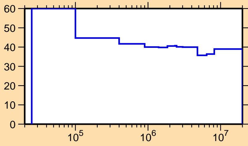
\Delta\sigma/\sigma vs. E for ^{83}\text{Zr}(n,n_1)
