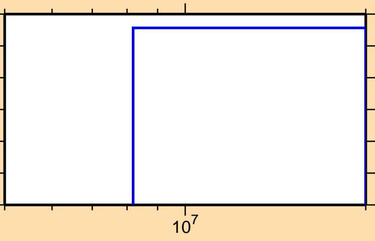
\sigma vs. E for ^{83}\text{Zr}(n,t)
