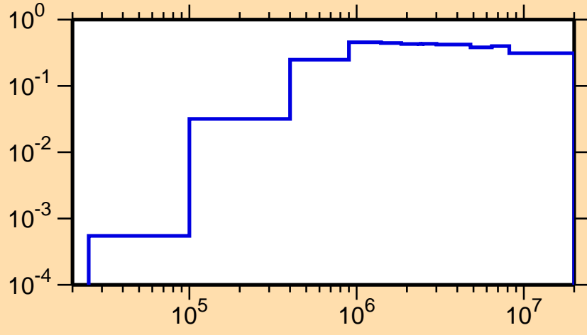
\sigma vs. E for ^{83}\text{Zr}(n,\text{inel.})
