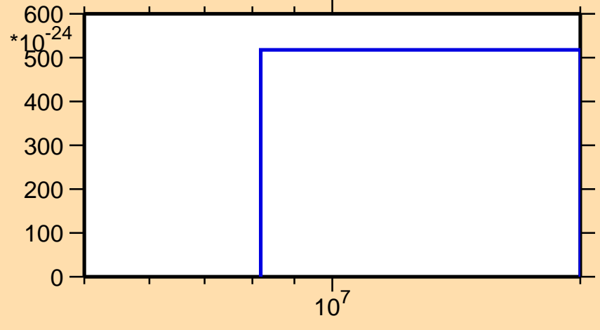
\sigma vs. E for ^{83}\text{Zr}(n,\text{nt})
