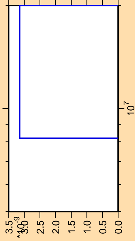
\Delta\sigma/\sigma vs. E for ^{83}\text{Zr}(n,\text{nt})
