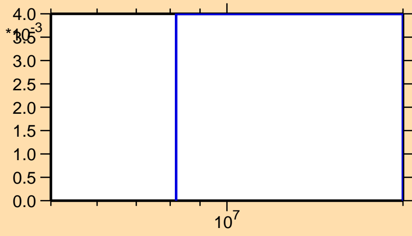
\sigma vs. E for ^{83}\text{Zr}(n,2n)
