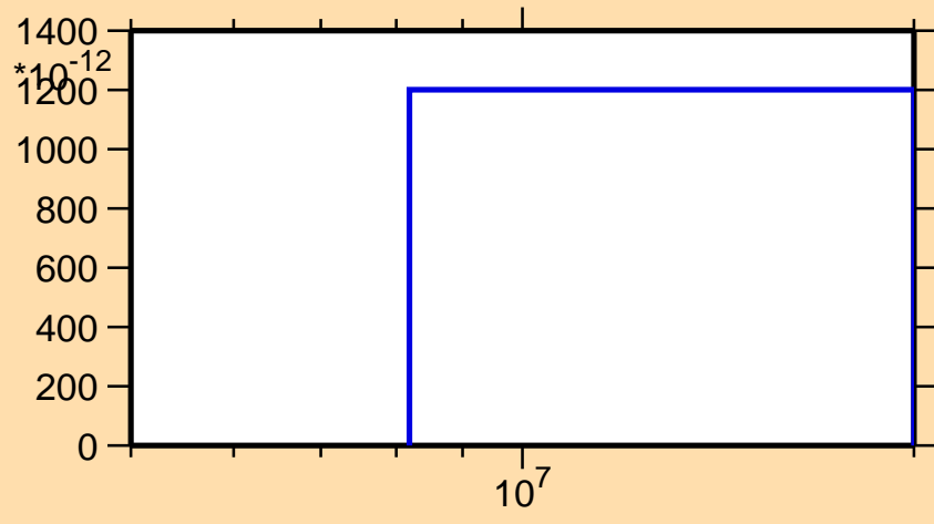
\sigma vs. E for ^{83}\text{Zr}(\text{mt } 45)
