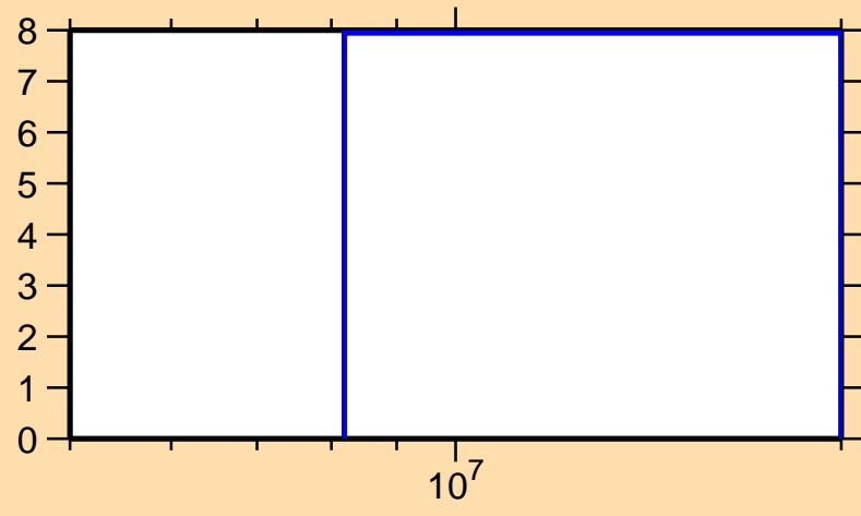
\Delta\sigma/\sigma vs. E for ^{83}\text{Zr}(n,\text{el.})
