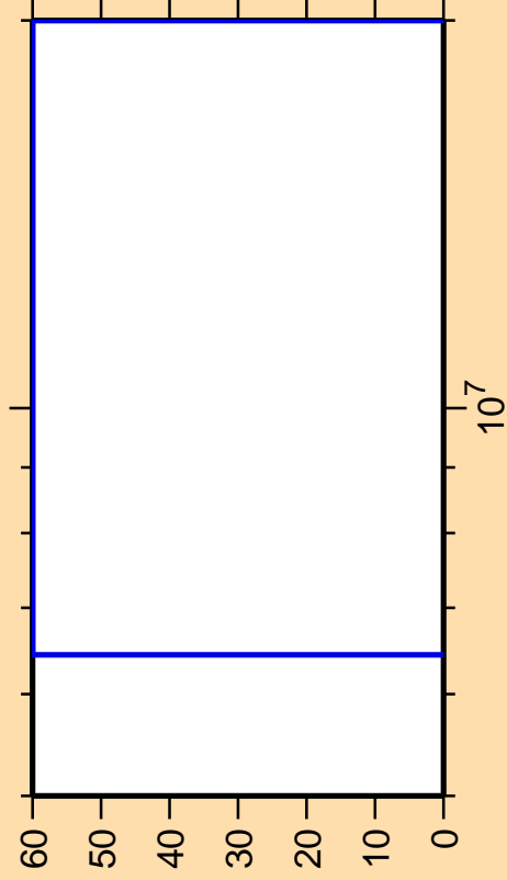
\Delta\sigma/\sigma vs. E for ^{83}\text{Zr}(n,n\alpha)
