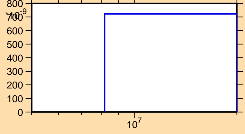
\sigma vs. E for ^{83}\text{Zr}(n,\text{pt})
