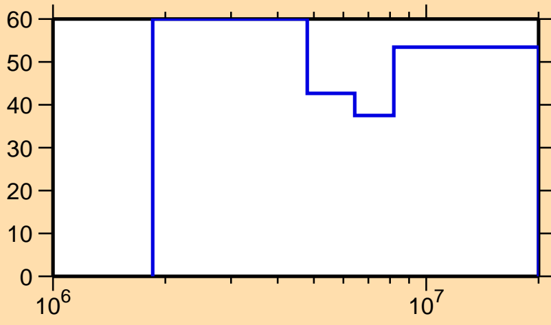
\Delta\sigma/\sigma vs. E for ^{83}\text{Zr}(n,n\text{cont.})
