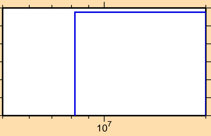
\sigma vs. E for ^{83}\text{Zr}(n,\text{pd})
