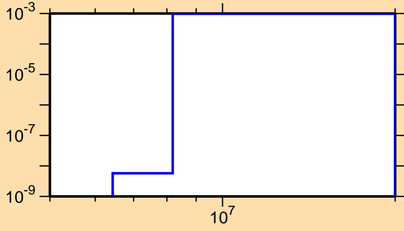
\sigma vs. E for ^{83}\text{Zr}(n,n\alpha)
