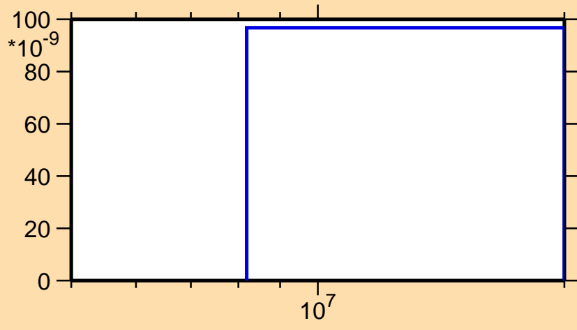
\sigma vs. E for ^{83}\text{Zr}(n,2np)
