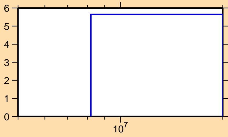
\Delta\sigma/\sigma vs. E for ^{83}\text{Zr}(n,\text{tot.})
