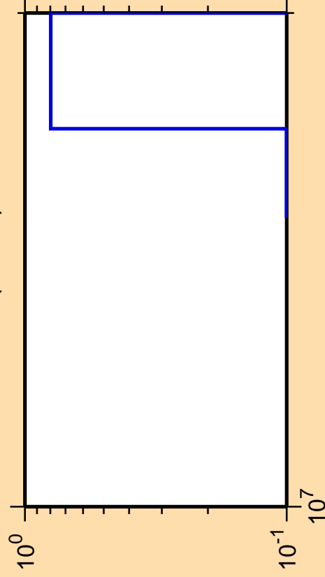
\Delta\sigma/\sigma vs. E for ^{84}\text{Zr} (mt 34)
