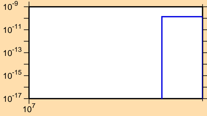
\sigma vs. E for ^{84}\text{Zr}(n,\text{nd})
