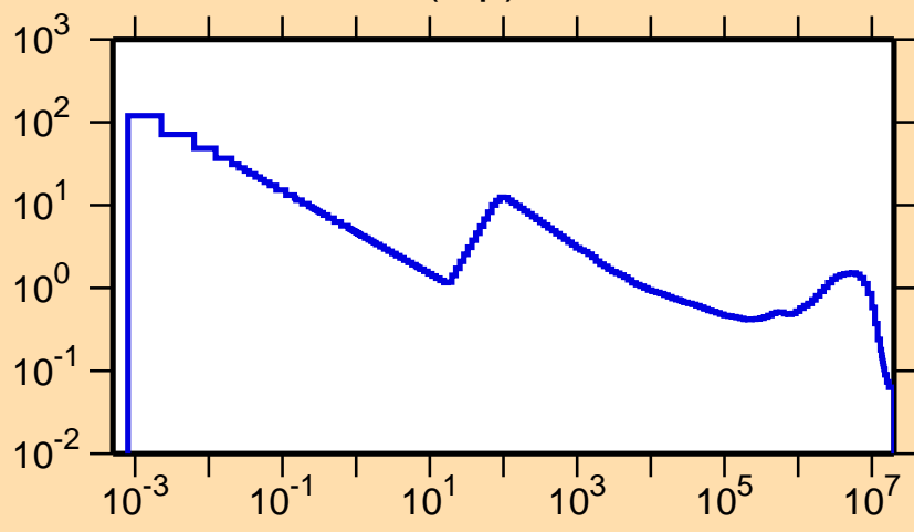
\sigma vs. E for ^{84}\text{Zr}(n,p)
