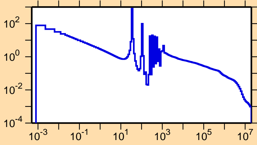
\sigma vs. E for ^{84}\text{Zr}(n,\gamma)
