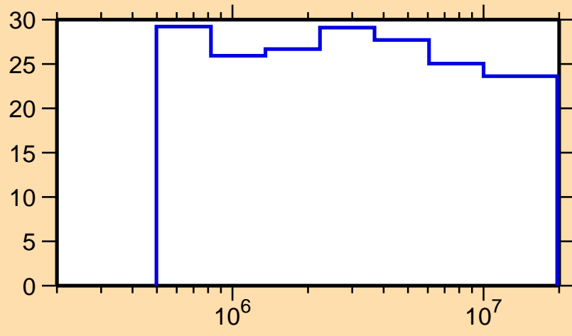
\Delta\sigma/\sigma vs. E for ^{84}\text{Zr}(n,n_1)
