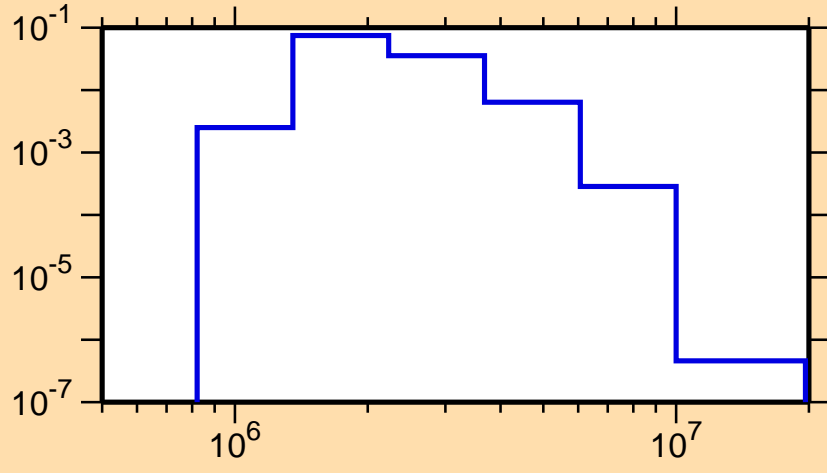
\sigma vs. E for ^{84}\text{Zr}(n,n_3)
