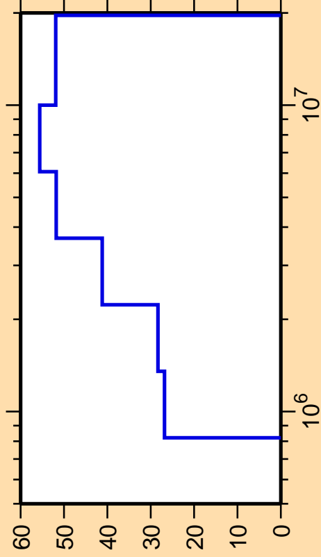
\Delta\sigma/\sigma vs. E for ^{84}\text{Zr}(n,n_3)
