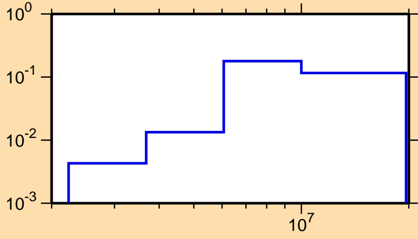
\sigma vs. E for ^{84}\text{Zr}(n,n\text{cont.})
