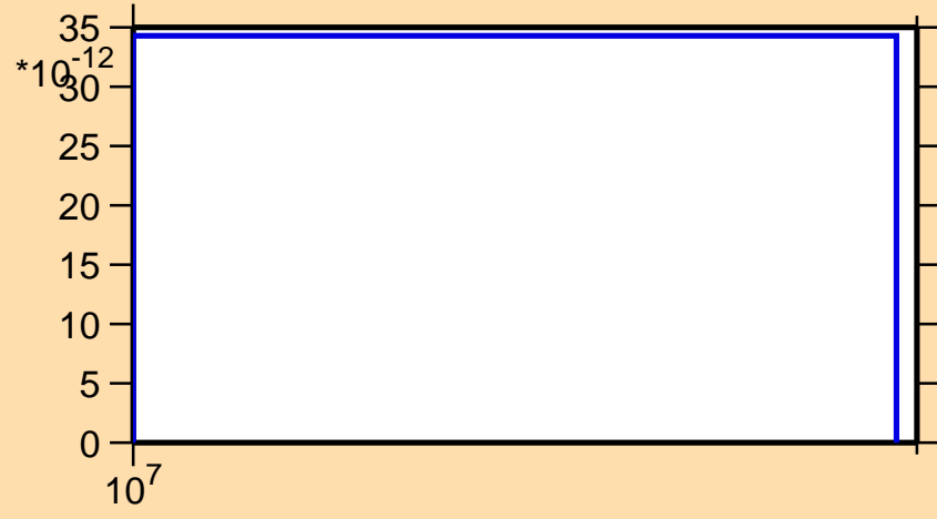
\sigma vs. E for ^{84}\text{Zr} (mt 45)
