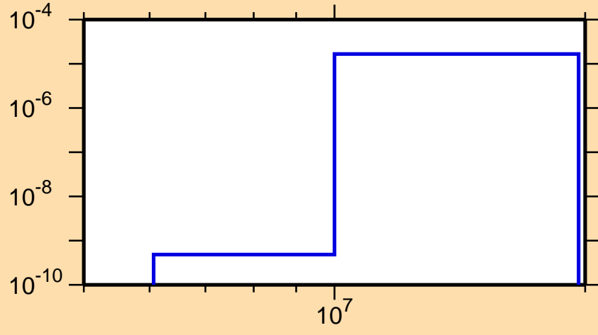
\sigma vs. E for ^{84}\text{Zr}(n,\text{He}3)
