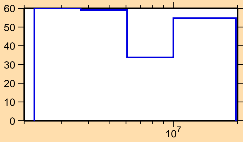
\Delta\sigma/\sigma vs. E for ^{84}\text{Zr}(n,n\text{cont.})
