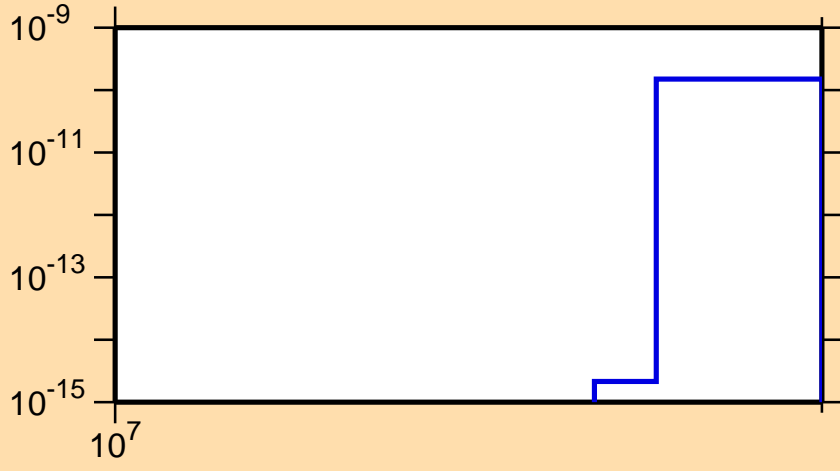
\sigma vs. E for ^{85}\text{Zr} (mt 45)
