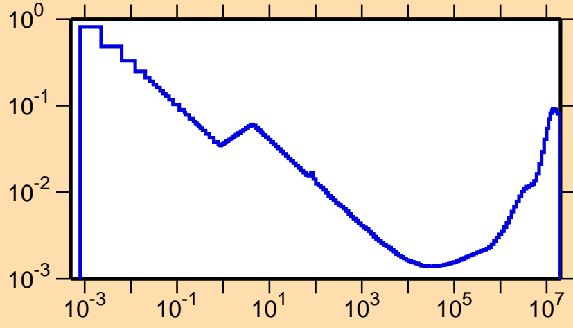
\sigma vs. E for ^{85}\text{Zr}(n,\alpha)
