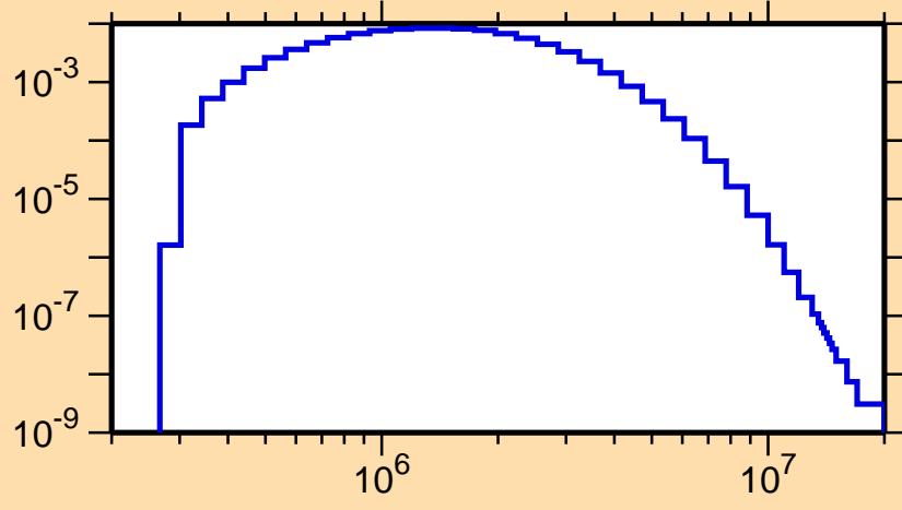
\sigma vs. E for ^{85}\text{Zr}(n,n_2)
