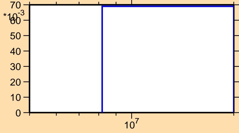
\sigma vs. E for ^{85}\text{Zr}(n,2n)
