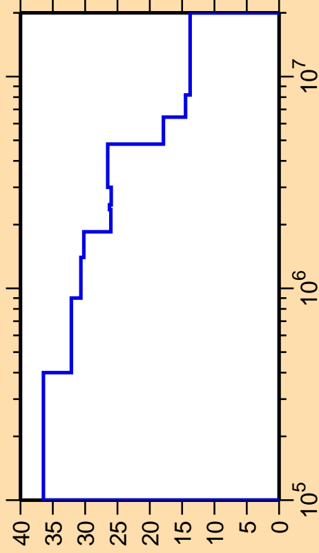
\Delta\sigma/\sigma vs. E for ^{85}\text{Zr}(n,n_2)
