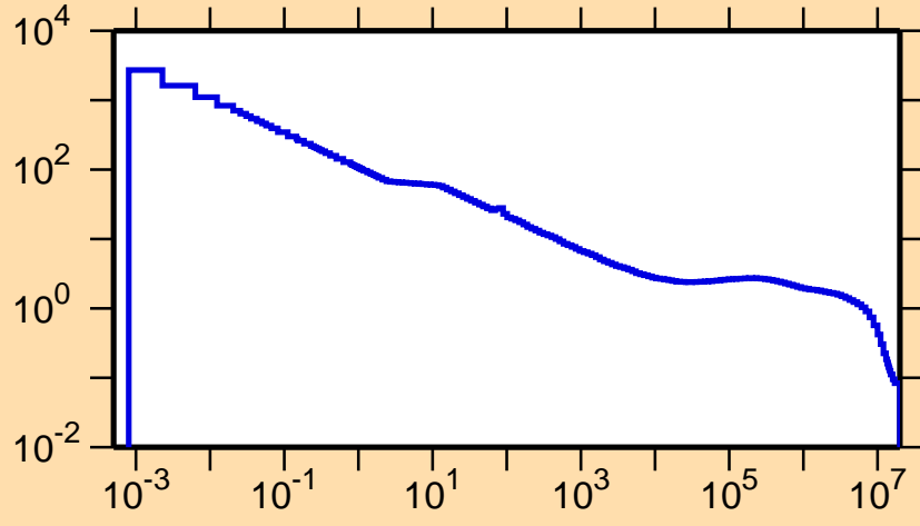
\sigma vs. E for ^{85}\text{Zr}(n,p)
