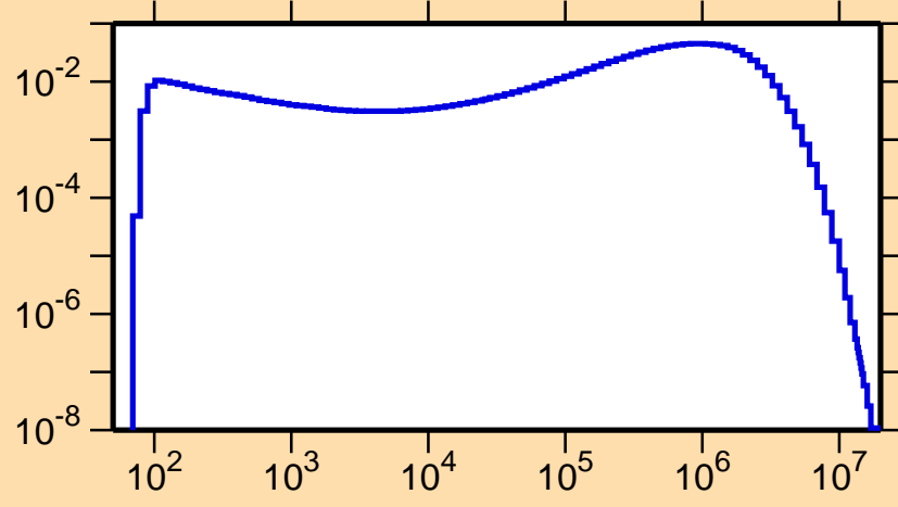
\sigma vs. E for ^{85}\text{Zr}(n,n_1)
