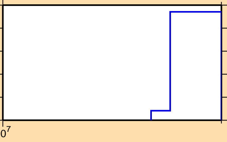
\sigma vs. E for ^{85}\text{Zr} (mt 45)
