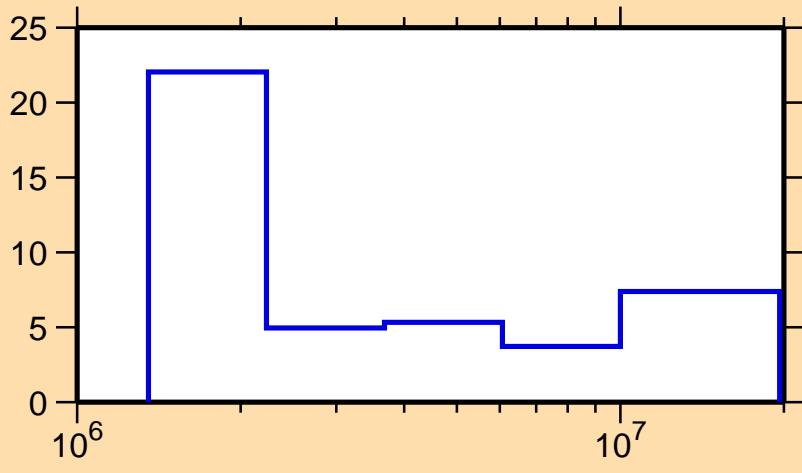
\Delta\sigma/\sigma vs. E for ^{85}\text{Zr}(n, el.)
