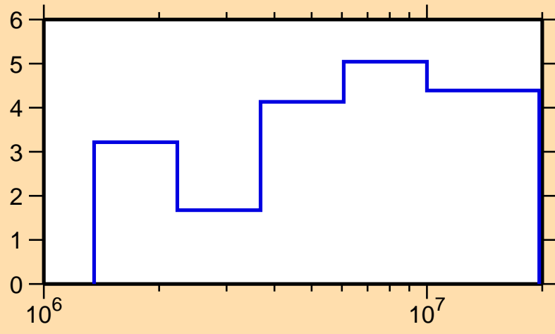
\Delta\sigma/\sigma vs. E for ^{85}\text{Zr}(n,n\text{onel.})
