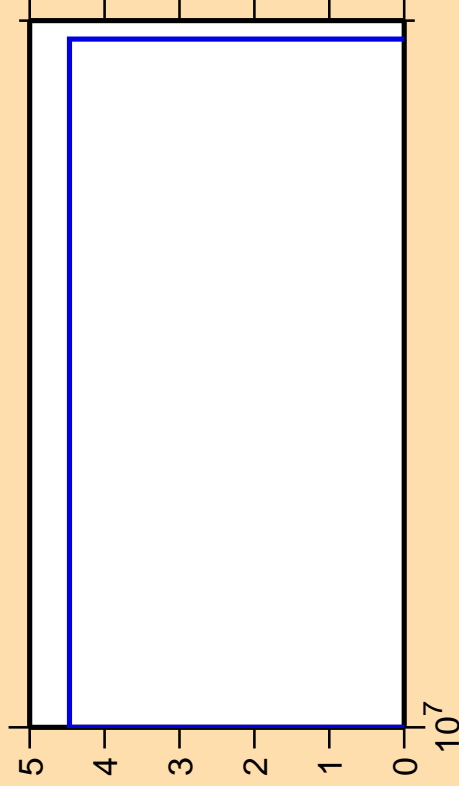
\Delta\sigma/\sigma vs. E for ^{85}\text{Zr}(n,2n\alpha)
