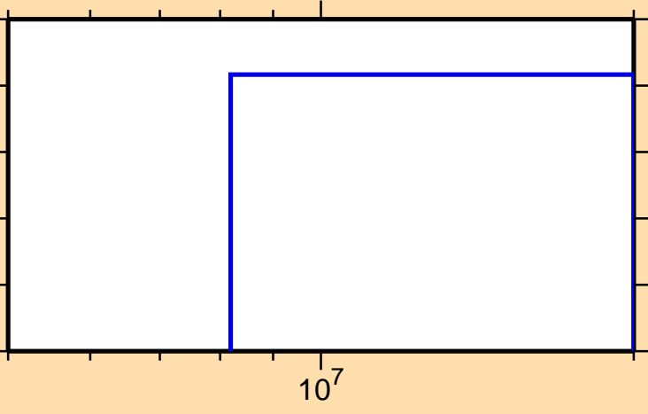
\sigma vs. E for ^{85}\text{Zr} (mt 45)
