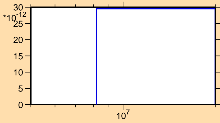
\sigma vs. E for ^{85}\text{Zr}(\text{mt } 34)
