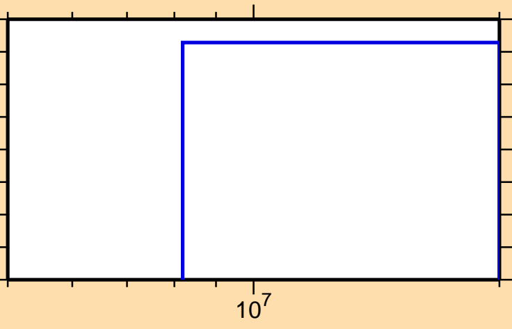
\sigma vs. E for ^{85}\text{Zr}(n,\text{pt})
