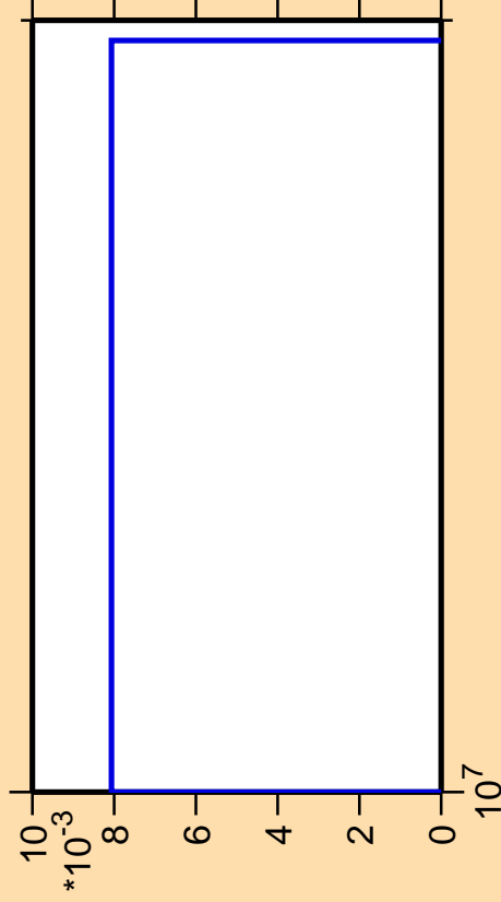
\Delta\sigma/\sigma vs. E for ^{86}\text{Zr} (mt 45)
