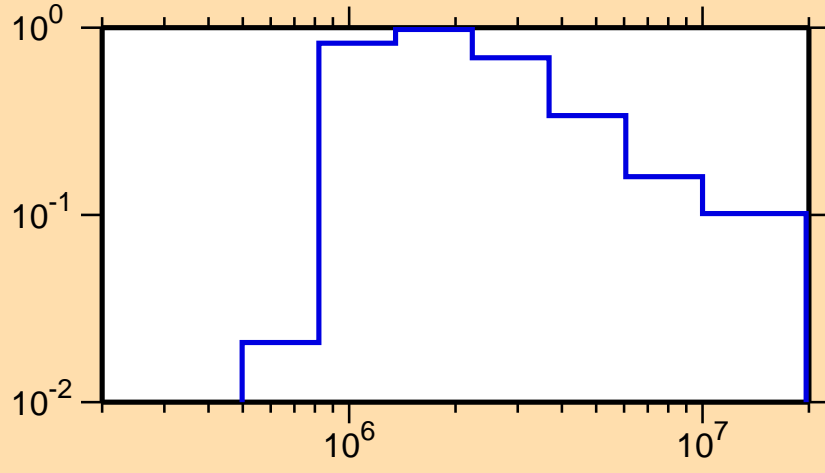
\sigma vs. E for ^{86}\text{Zr}(n,n_1)
