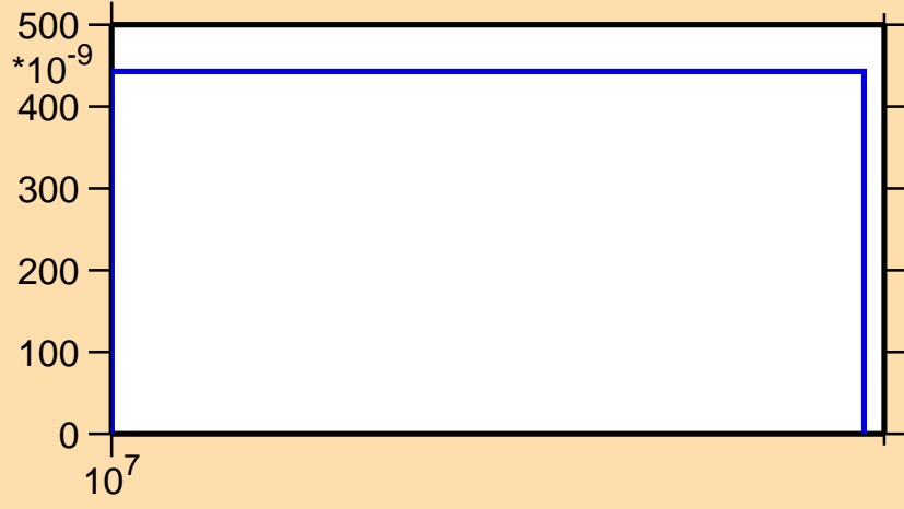
\sigma vs. E for ^{86}\text{Zr}(n,pd)
