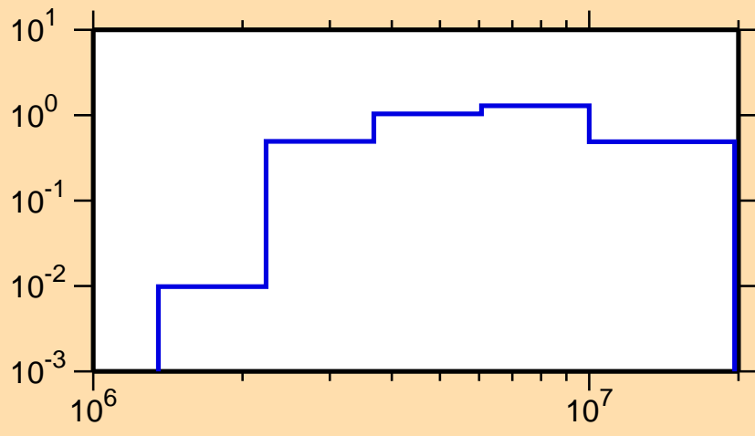
\sigma vs. E for ^{87}\text{Zr}(n,n\text{cont.})
