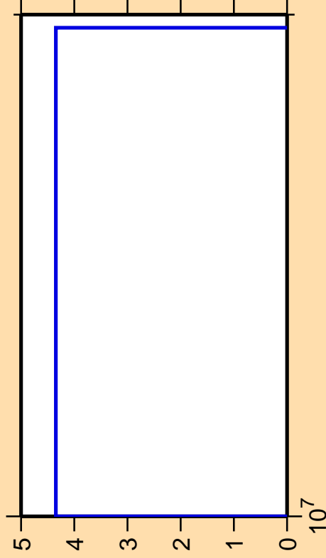
\Delta\sigma/\sigma vs. E for ^{87}\text{Zr}(n,2n\alpha)
