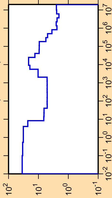
\Delta\sigma/\sigma vs. E for ^{87}\text{Zr}(n,\text{nonel.})
