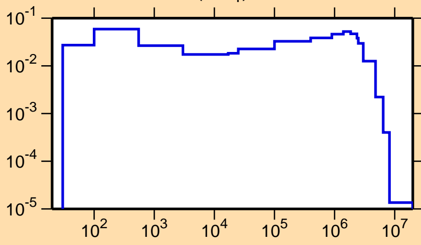
\sigma vs. E for ^{87}\text{Zr}(n,n_1)
