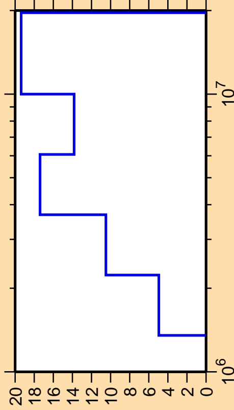
\Delta\sigma/\sigma vs. E for ^{88}\text{Zr}(n,n_3)
