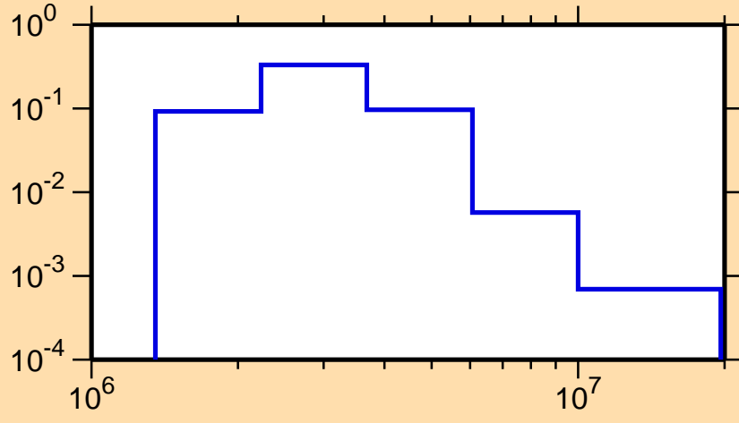
\sigma vs. E for ^{88}\text{Zr}(n,n_3)
