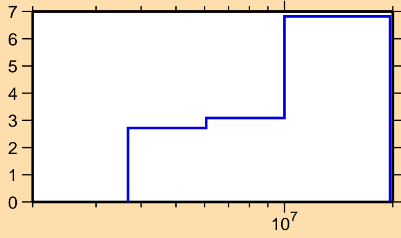
\Delta\sigma/\sigma vs. E for ^{88}\text{Zr}(n,inel.)
