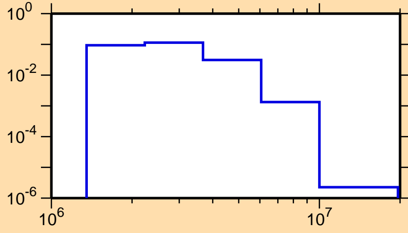
\sigma vs. E for ^{88}\text{Zr}(n,n_2)
