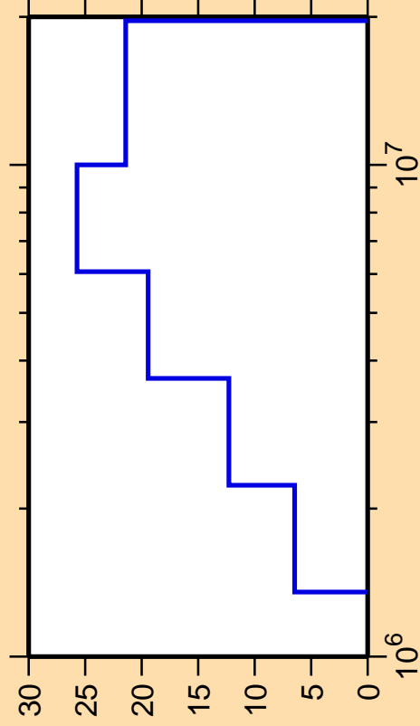
\Delta\sigma/\sigma vs. E for ^{88}\text{Zr}(n,n_2)
