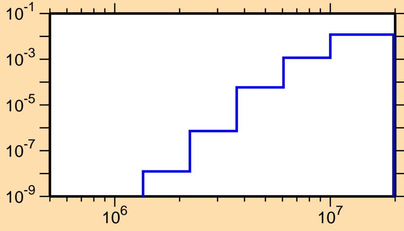
\sigma vs. E for ^{88}\text{Zr}(n,\alpha)
