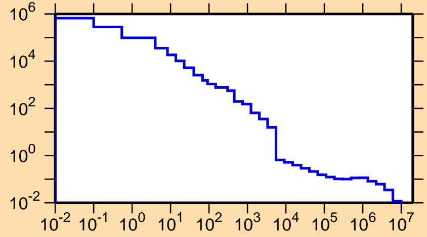
\sigma vs. E for ^{88}\text{Zr}(n,\gamma)
