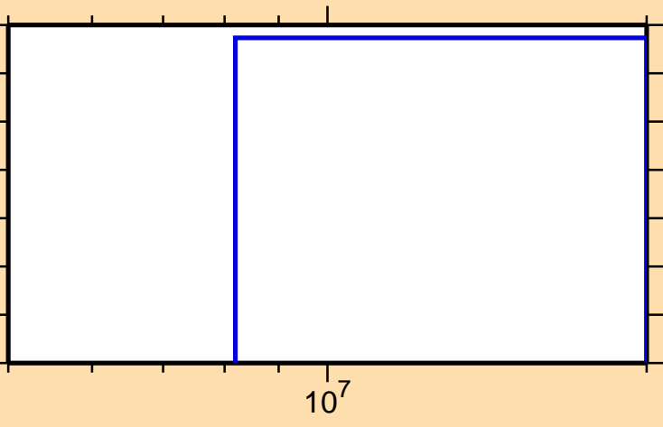
\sigma vs. E for ^{88}\text{Zr}(n,p\alpha)
