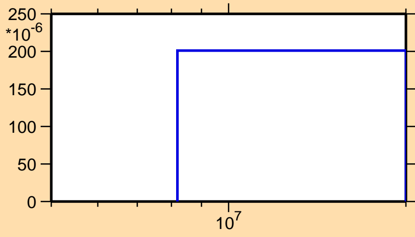
\sigma vs. E for ^{88}\text{Zr}(n,n\alpha)
