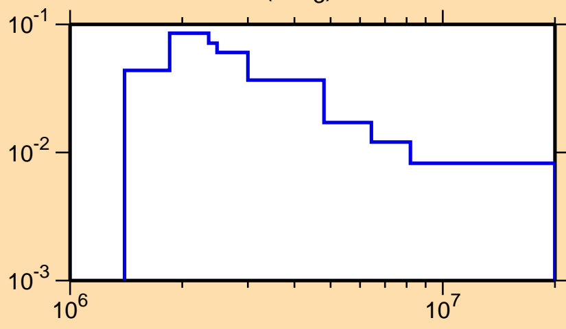
\sigma vs. E for ^{89}\text{Zr}(n,n_3)
