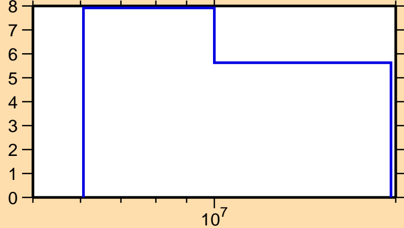
\Delta\sigma/\sigma vs. E for ^{89}\text{Zr}(n,2n)
