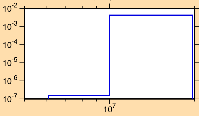
\sigma vs. E for ^{90}\text{Zr}(n,d)
