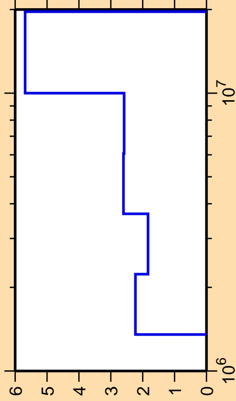
\Delta\sigma/\sigma vs. E for ^{90}\text{Zr}(n,\text{inel.})
