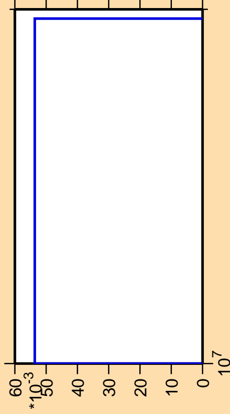
\Delta\sigma/\sigma vs. E for ^{90}\text{Zr}(n,nd)
