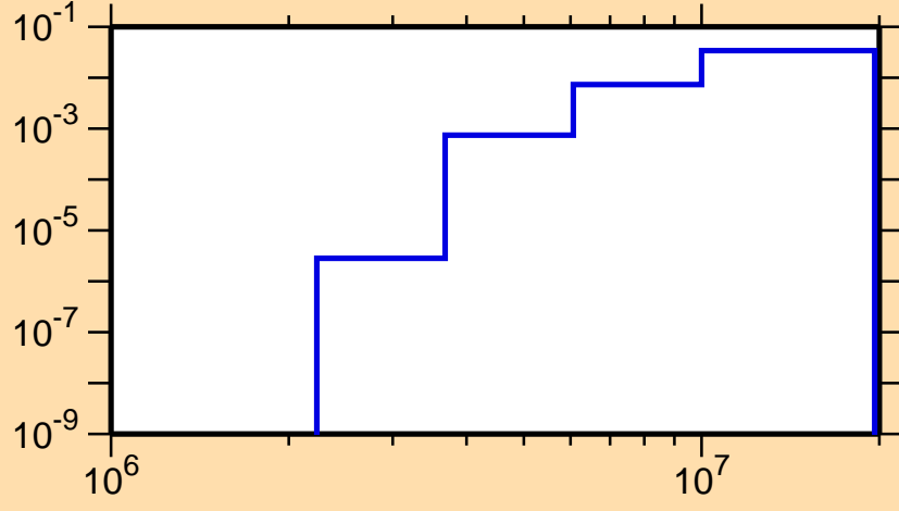
\sigma vs. E for ^{90}\text{Zr}(n,p)
