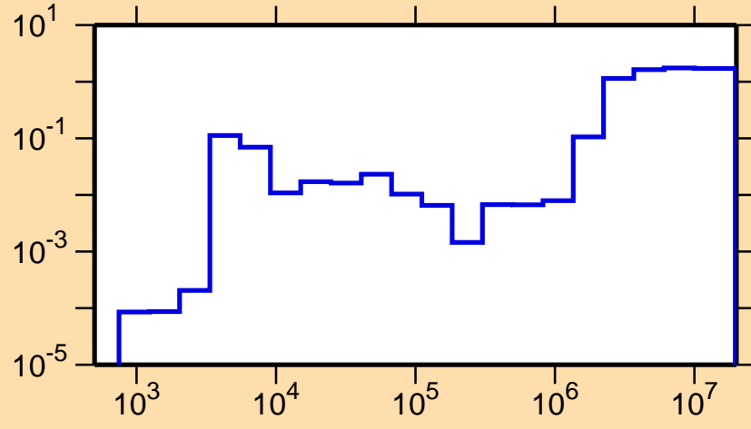
\sigma vs. E for ^{90}\text{Zr}(n,\text{nonel.})
