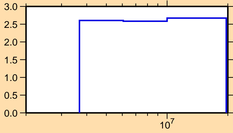
\Delta\sigma/\sigma vs. E for ^{90}\text{Zr}(n,n\text{onel.})
