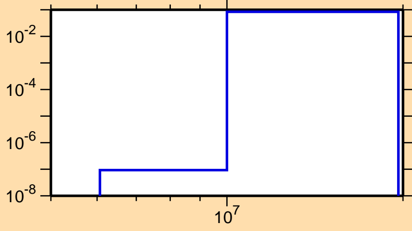
\sigma vs. E for ^{90}\text{Zr}(n,np)
