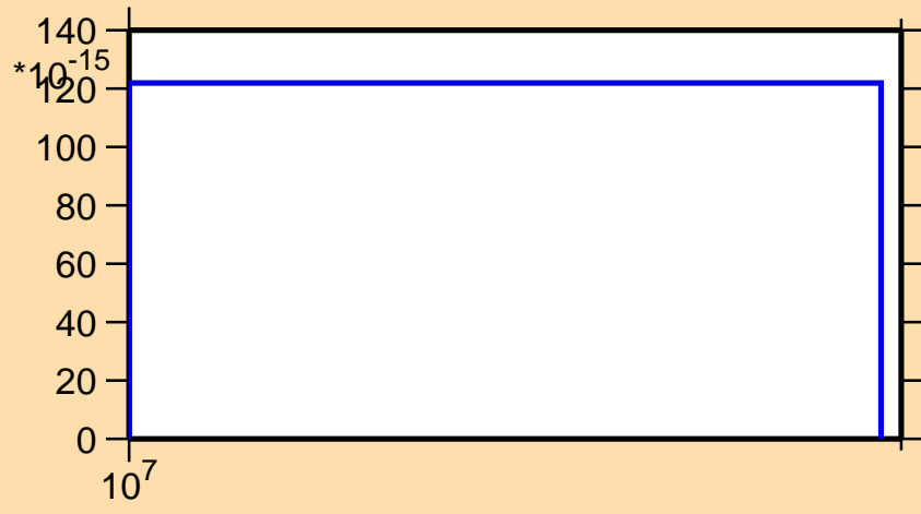
\sigma vs. E for ^{90}\text{Zr}(n,nd)
