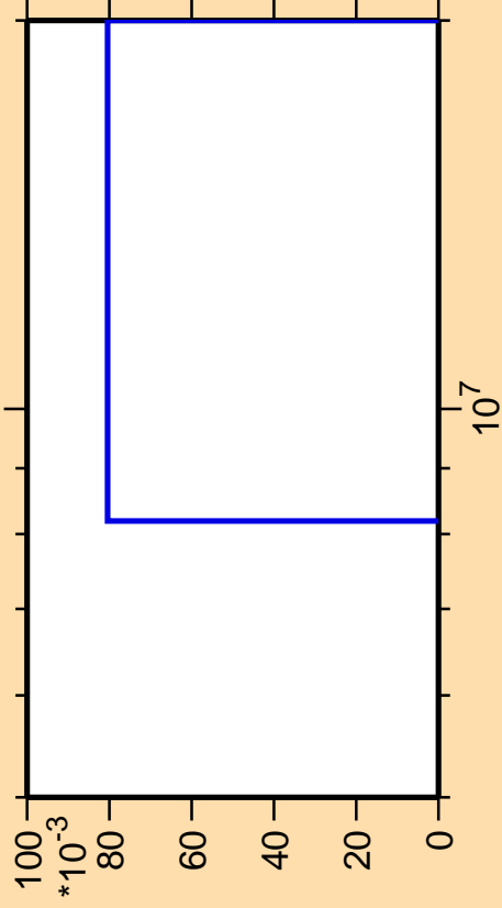
\Delta\sigma/\sigma vs. E for ^{90}\text{Zr}(n,\text{nd})
