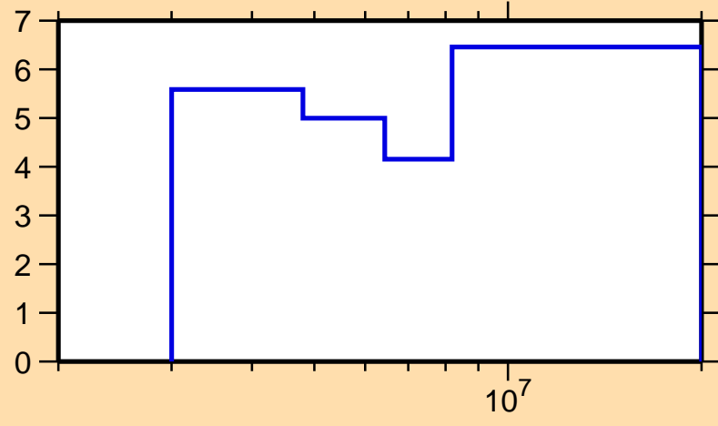
\Delta\sigma/\sigma vs. E for ^{90}\text{Zr}(n,n\text{cont.})
