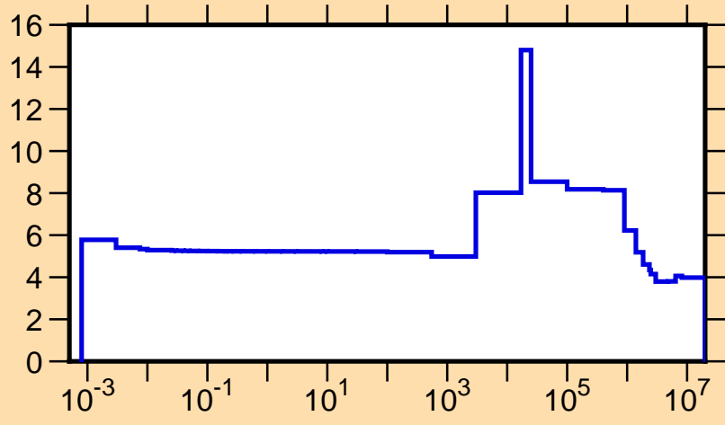
\sigma vs. E for ^{90}\text{Zr}(n,\text{tot.})
