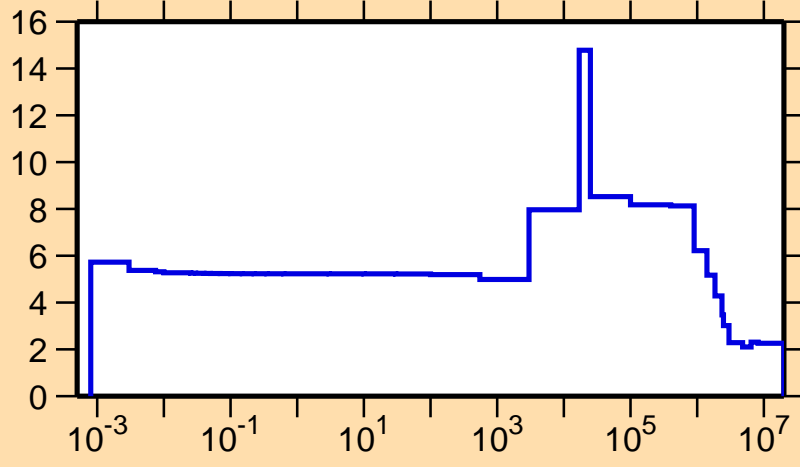
\sigma vs. E for ^{90}\text{Zr}(n,\text{el.})
