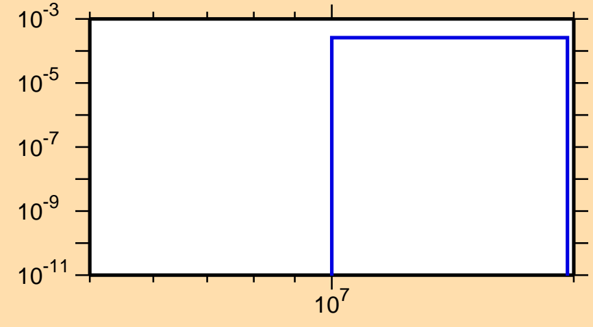
\sigma vs. E for ^{91}\text{Zr}(n,n\alpha)
