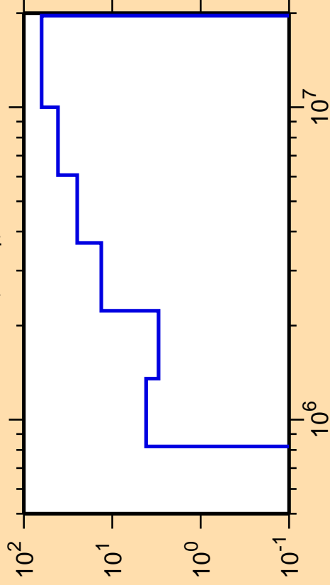
\Delta\sigma/\sigma vs. E for ^{91}\text{Zr}(n,n_1)
