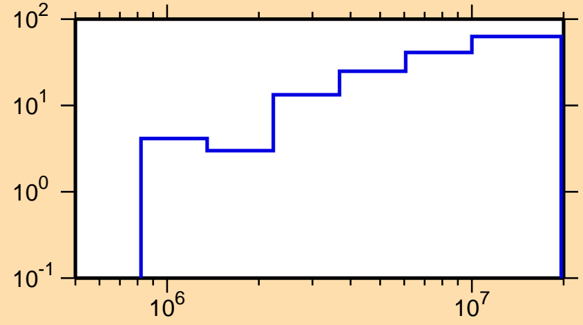
\Delta\sigma/\sigma vs. E for ^{91}\text{Zr}(n,n_1)
