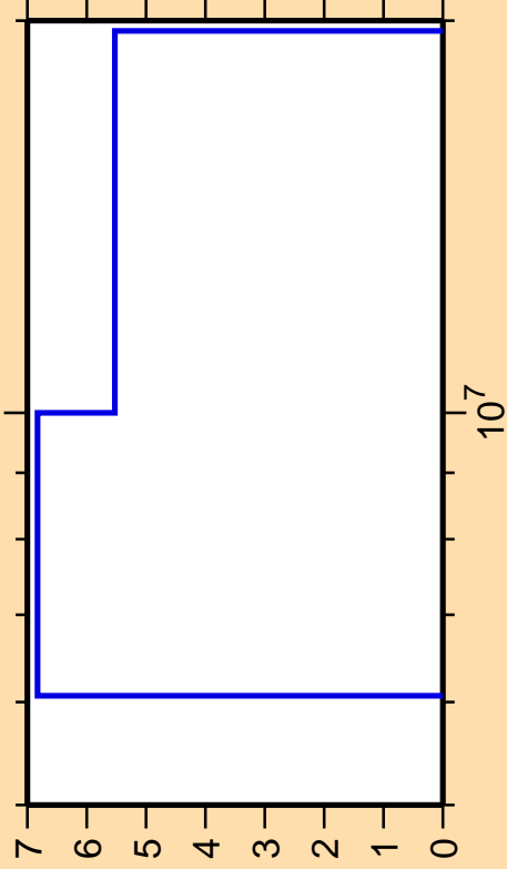
\Delta\sigma/\sigma vs. E for ^{91}\text{Zr}(n,2n)
