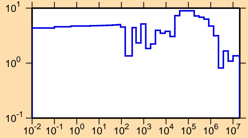
\Delta\sigma/\sigma vs. E for ^{91}\text{Zr}(n,\text{tot.})
