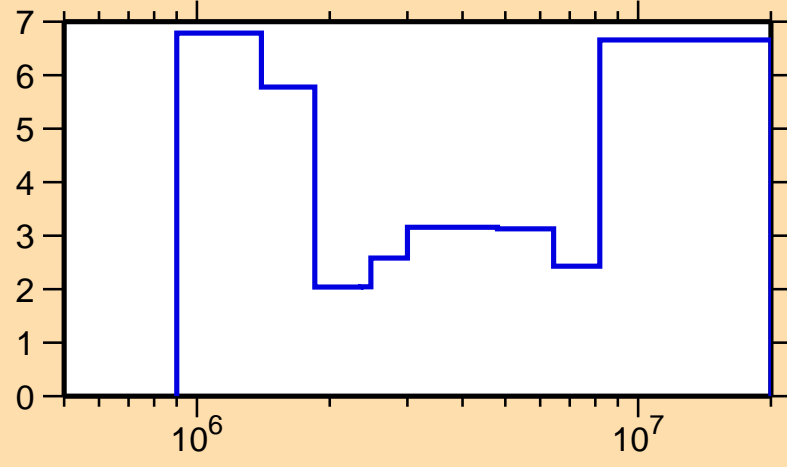
\Delta\sigma/\sigma vs. E for ^{91}\text{Zr}(n,\text{inel.})
