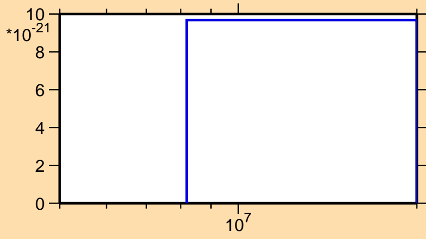
\sigma vs. E for ^{91}\text{Zr}(n,nt)
