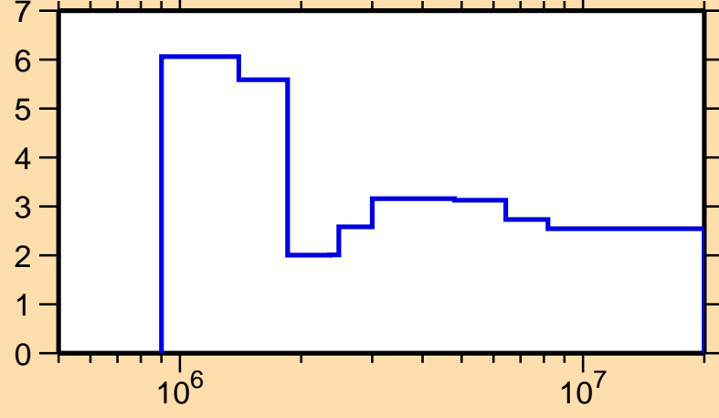
\Delta\sigma/\sigma vs. E for ^{91}\text{Zr}(n,\text{nonel.})
