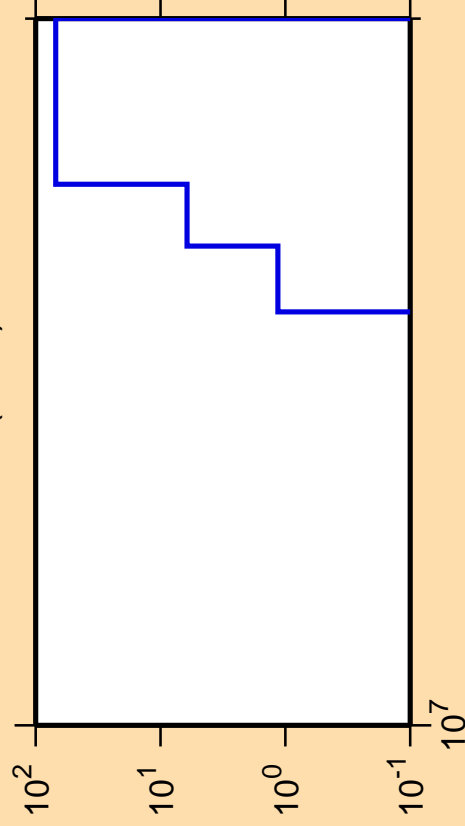
\Delta\sigma/\sigma vs. E for ^{92}\text{Zr}(n,nd)
