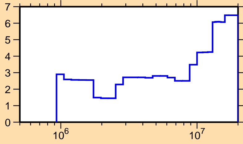
\Delta\sigma/\sigma vs. E for ^{92}\text{Zr}(n,\text{inel.})
