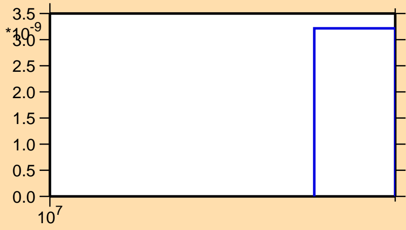
\sigma vs. E for ^{92}\text{Zr}(n,2np)
