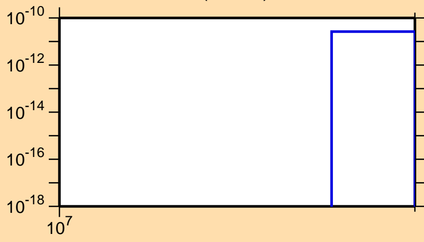
\sigma vs. E for ^{92}\text{Zr}(n,2n\alpha)
