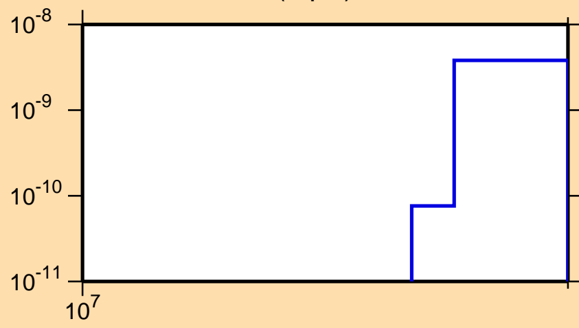
\sigma vs. E for ^{92}\text{Zr}(n,p\alpha)
