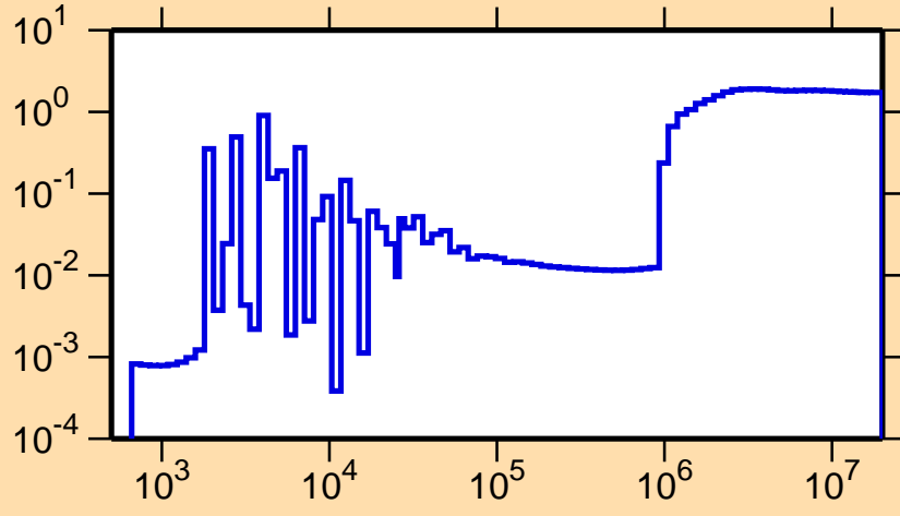
\sigma vs. E for ^{92}\text{Zr}(n,\text{nonel.})
