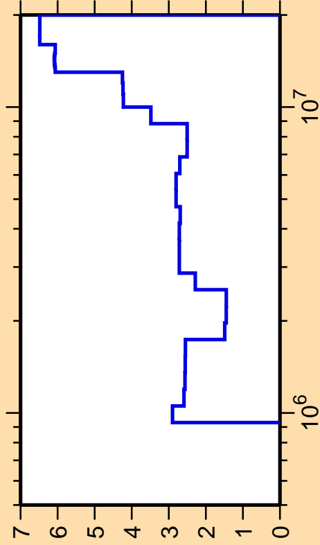
\Delta\sigma/\sigma vs. E for ^{92}\text{Zr}(n,\text{inel.})
