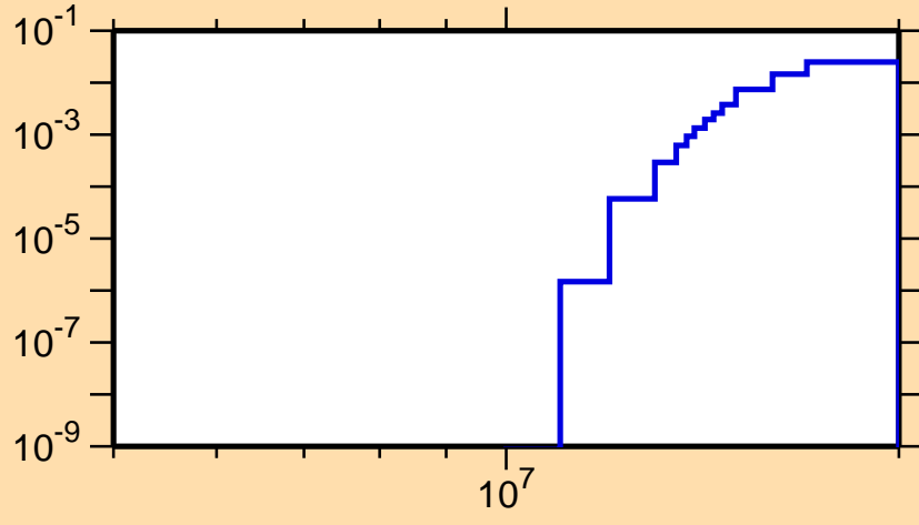
\sigma vs. E for ^{92}\text{Zr}(n,np)
