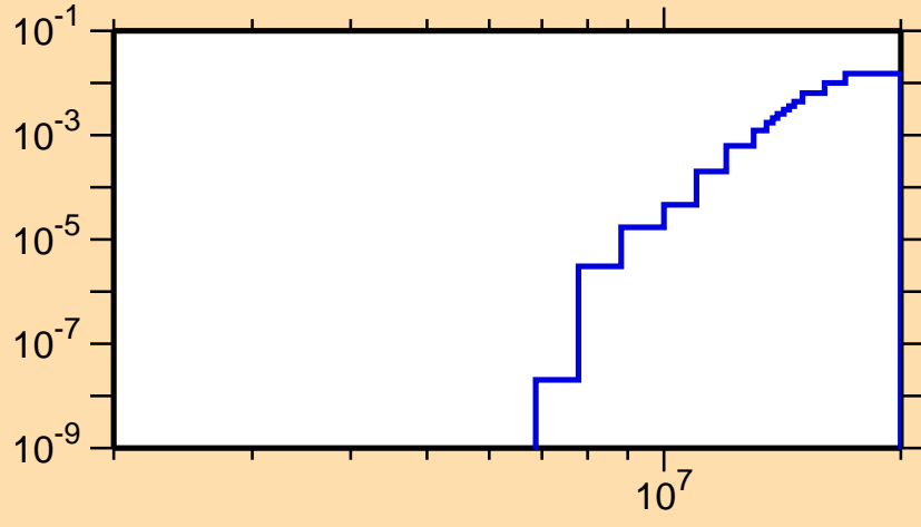
\sigma vs. E for ^{92}\text{Zr}(n,n\alpha)
