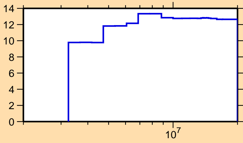
\Delta\sigma/\sigma vs. E for ^{92}\text{Zr}(n, n_1)
