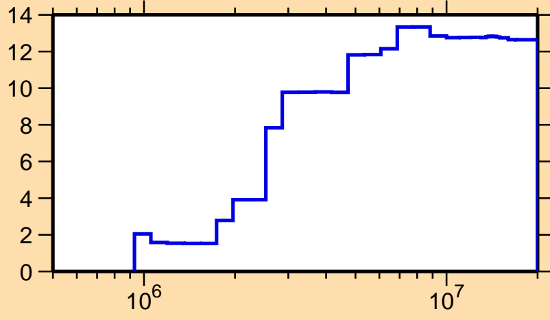
\Delta\sigma/\sigma vs. E for ^{92}\text{Zr}(n,n_1)
