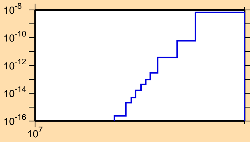
\sigma vs. E for ^{92}\text{Zr}(n,\text{He}3)
