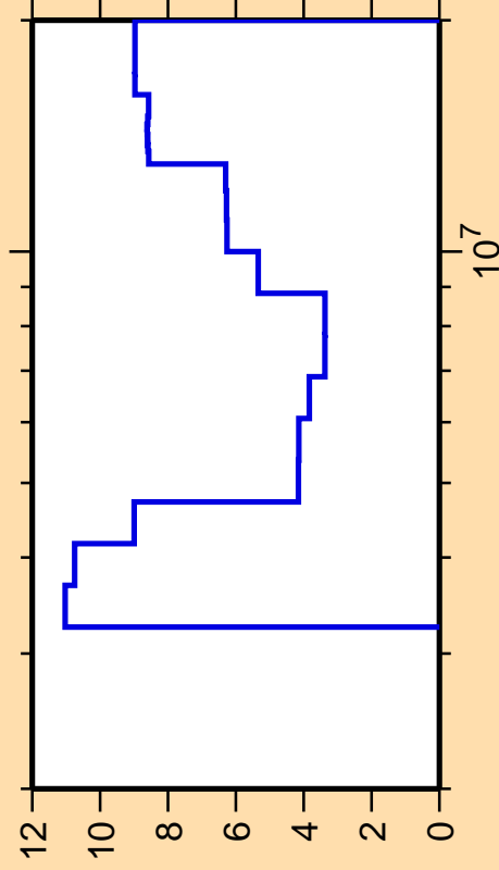
\Delta\sigma/\sigma vs. E for ^{92}\text{Zr}(n,\text{ncont.})
