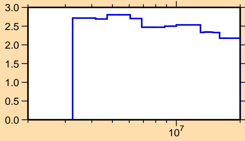
\Delta\sigma/\sigma vs. E for ^{92}\text{Zr}(n,n\text{onel.})
