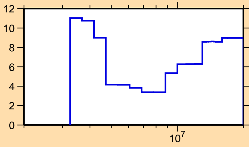
\Delta\sigma/\sigma vs. E for ^{92}\text{Zr}(n,n\text{cont.})
