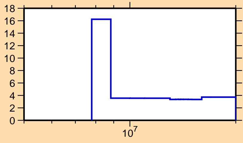
\Delta\sigma/\sigma vs. E for ^{92}\text{Zr}(n,2n)
