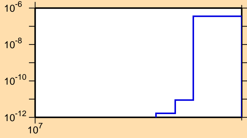
\sigma vs. E for ^{92}\text{Zr}(n,nd)
