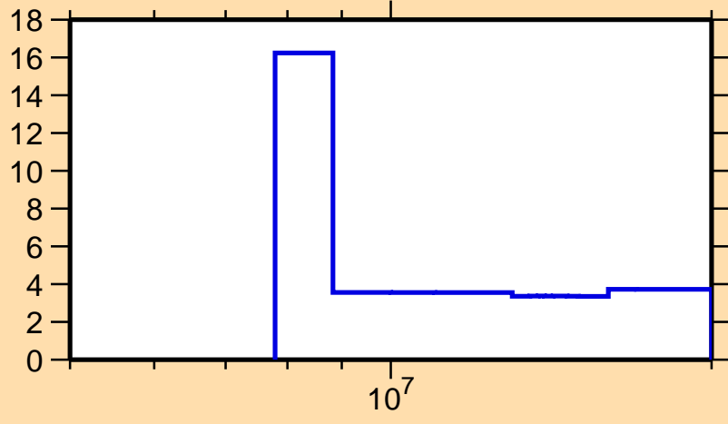
\Delta\sigma/\sigma vs. E for ^{92}\text{Zr}(n,2n)
