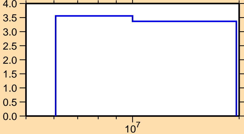
\Delta\sigma/\sigma vs. E for ^{92}\text{Zr}(n,2n)
