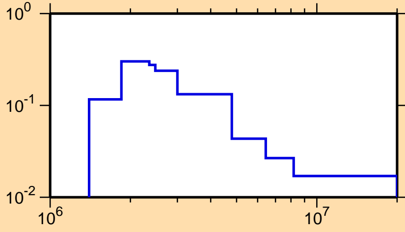
\sigma vs. E for ^{92}\text{Zr}(n,n_3)
