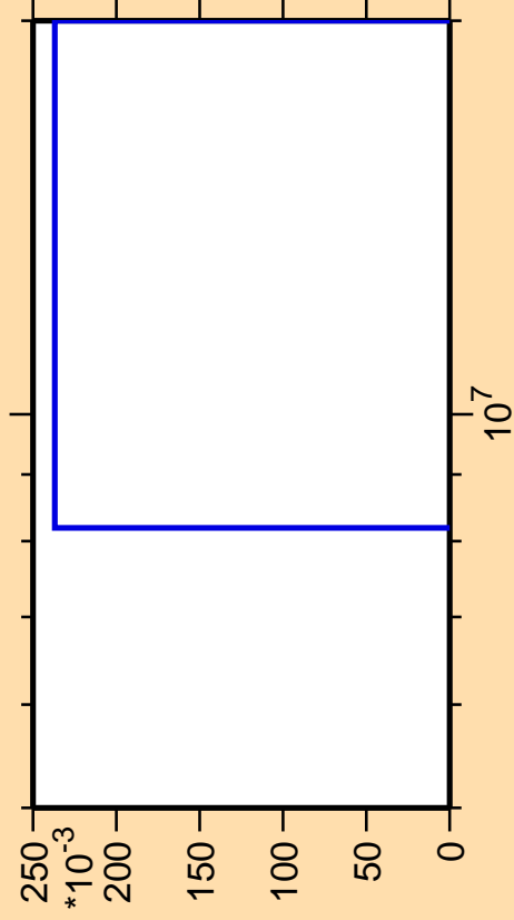
\Delta\sigma/\sigma vs. E for ^{92}\text{Zr}(n,2n\alpha)
