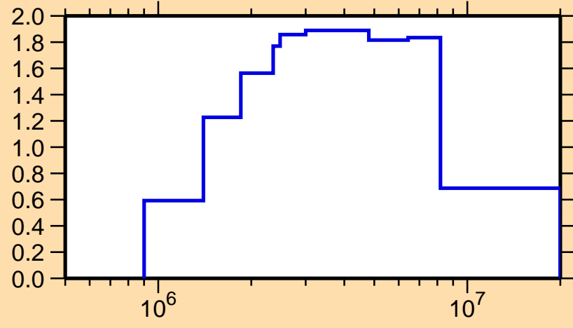
\sigma vs. E for ^{92}\text{Zr}(n,\text{inel.})
