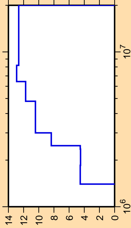
\Delta\sigma/\sigma vs. E for ^{92}\text{Zr}(n,n_3)
