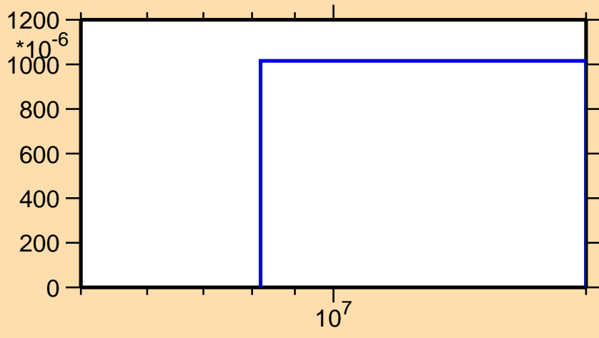
\sigma vs. E for ^{92}\text{Zr}(n,d)
