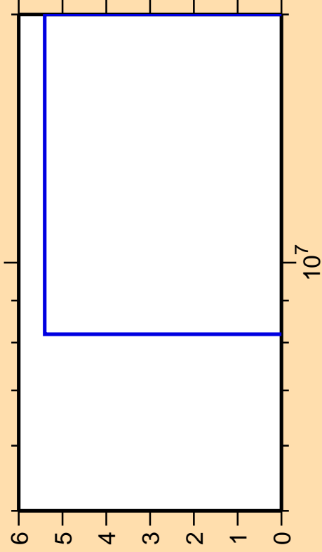
\Delta\sigma/\sigma vs. E for ^{92}\text{Zr}(n,n\text{cont.})
