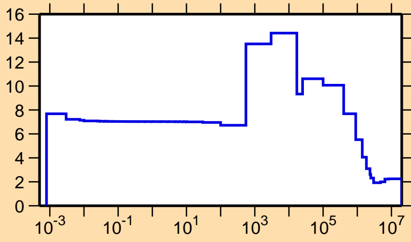
\sigma vs. E for ^{92}\text{Zr}(n,\text{el.})
