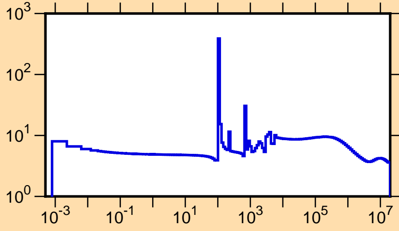
\sigma vs. E for ^{93}\text{Zr}(n,\text{tot.})
