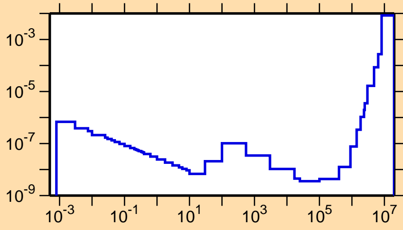
\sigma vs. E for ^{93}\text{Zr}(n,\alpha)
