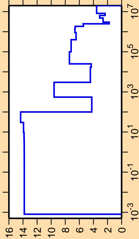
\Delta\sigma/\sigma vs. E for ^{93}\text{Zr}(n,\text{el.})
