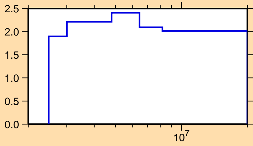
\Delta\sigma/\sigma vs. E for ^{93}\text{Zr}(n,n\text{onl.})
