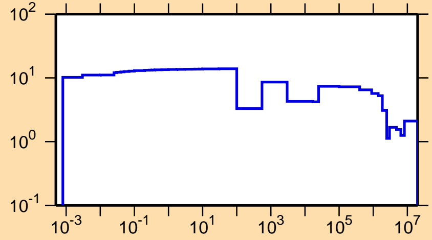
\Delta\sigma/\sigma vs. E for ^{93}\text{Zr}(n,\text{tot.})
