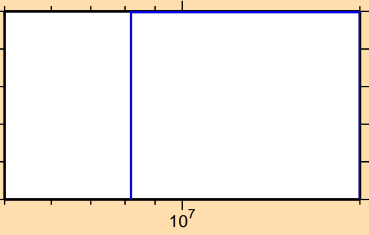
\sigma vs. E for ^{93}\text{Zr}(n,d)
