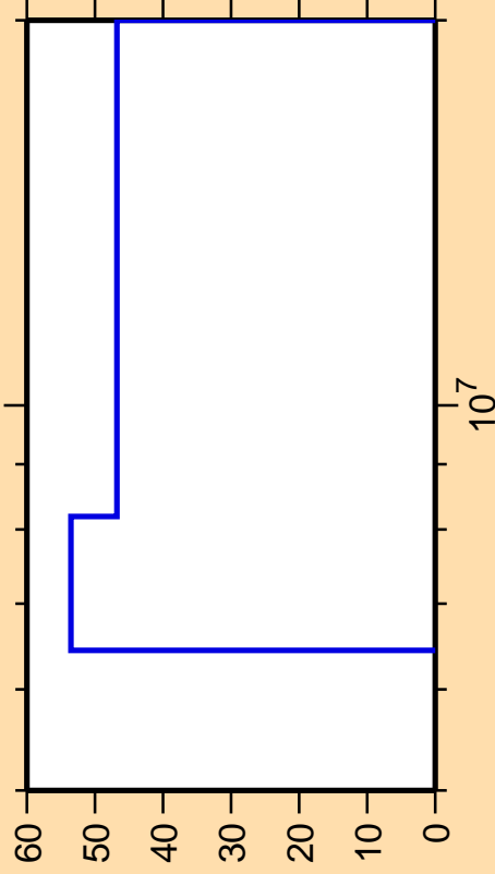
\Delta\sigma/\sigma vs. E for ^{93}\text{Zr}(n,\alpha)
