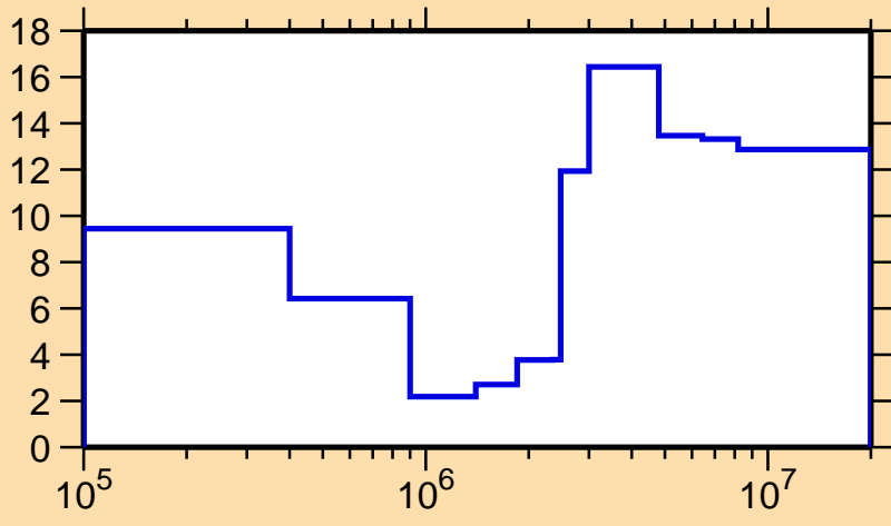
\Delta\sigma/\sigma vs. E for ^{93}\text{Zr}(n,n_1)
