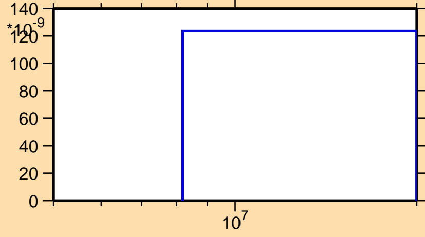
\sigma vs. E for ^{93}\text{Zr}(n,2n\alpha)
