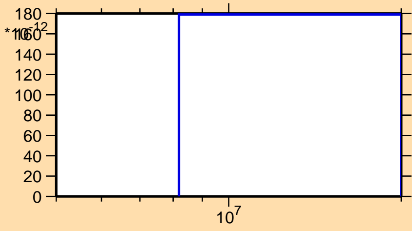
\sigma vs. E for ^{93}\text{Zr}(n,\text{He3})
