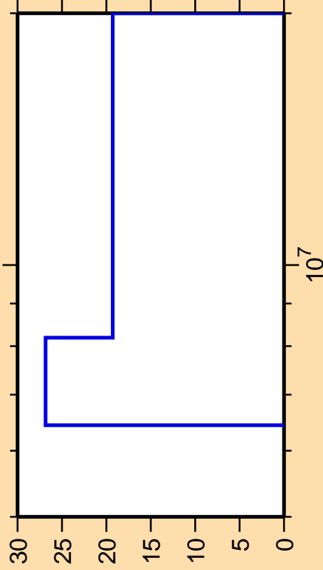
\Delta\sigma/\sigma vs. E for ^{93}\text{Zr}(n,p)
