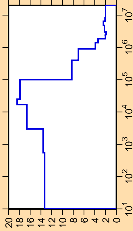
\Delta\sigma/\sigma vs. E for ^{93}\text{Zr}(n,\text{nonel.})
