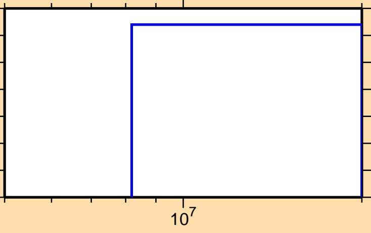
\sigma vs. E for ^{93}\text{Zr}(n,np)
