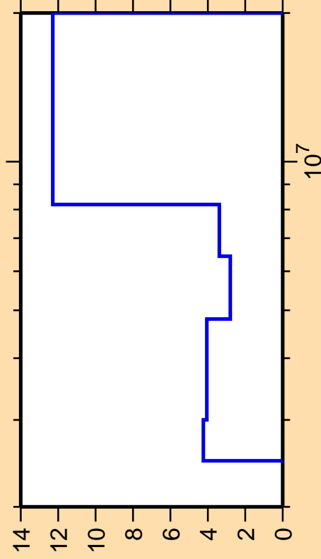
\Delta\sigma/\sigma vs. E for ^{93}\text{Zr}(n,\text{ncont.})
