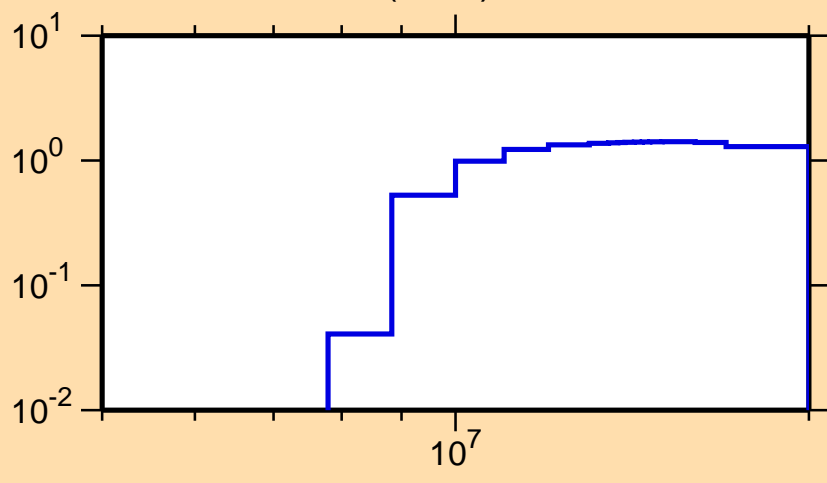
\sigma vs. E for ^{94}\text{Zr}(n,2n)
