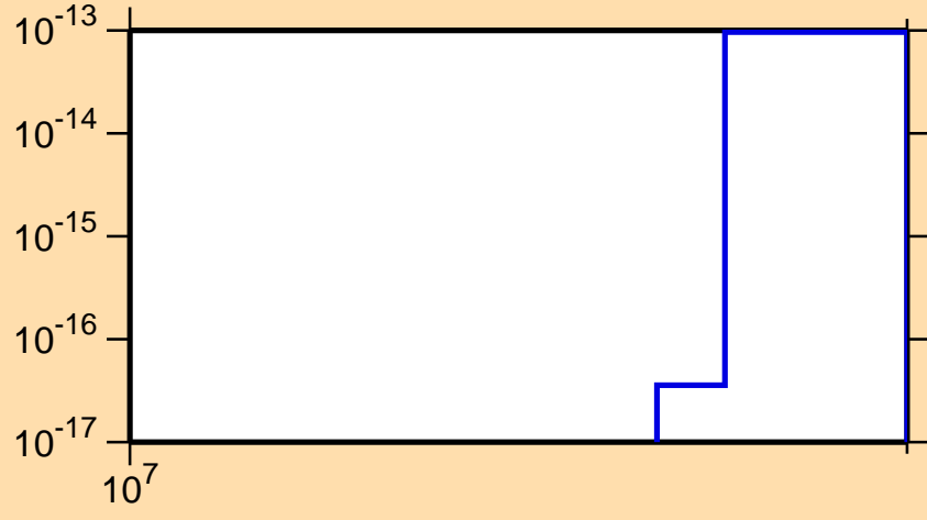
\sigma vs. E for ^{94}\text{Zr}(n,p\alpha)
