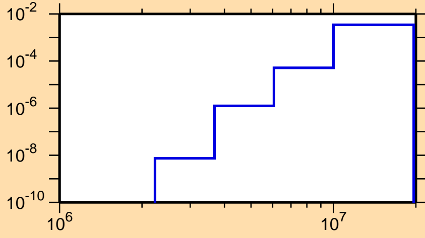
\sigma vs. E for ^{94}\text{Zr}(n,\alpha)
