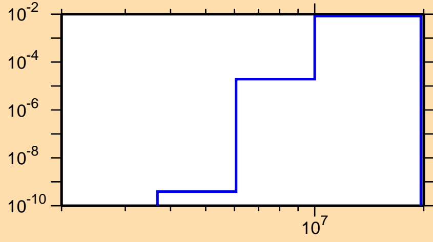
\sigma vs. E for ^{94}\text{Zr}(n,p)
