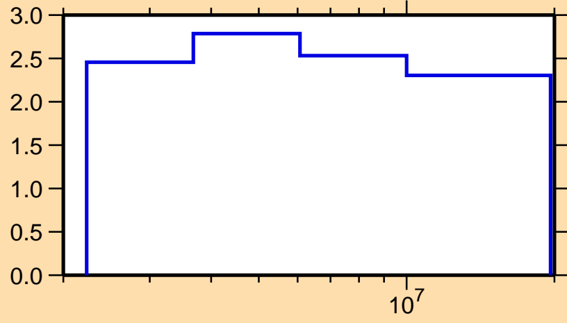
\Delta\sigma/\sigma vs. E for ^{94}\text{Zr}(n,n\text{onel.})
