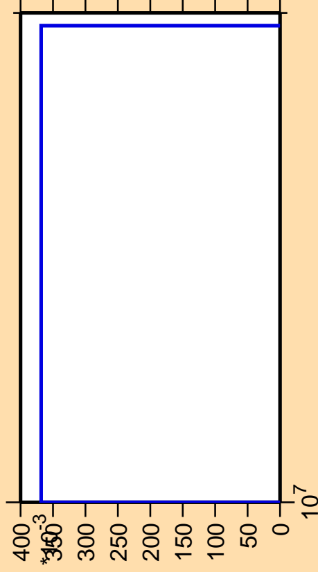
\Delta\sigma/\sigma vs. E for ^{94}\text{Zr}(n,2np)
