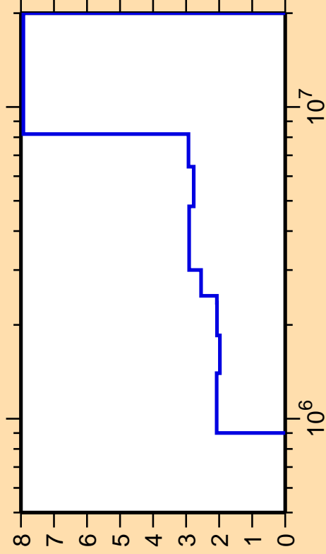
\Delta\sigma/\sigma vs. E for ^{94}\text{Zr}(n,\text{inel.})
