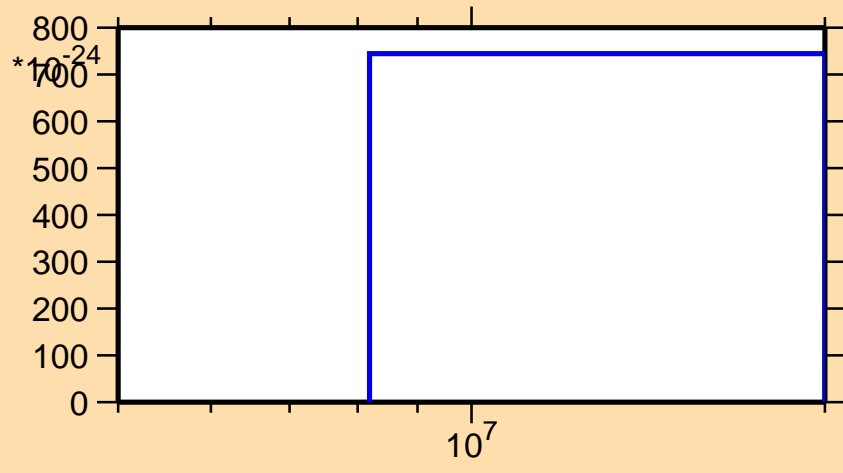
\sigma vs. E for ^{94}\text{Zr}(\text{mt } 34)
