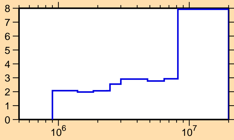
\Delta\sigma/\sigma vs. E for ^{94}\text{Zr}(n,\text{inel.})
