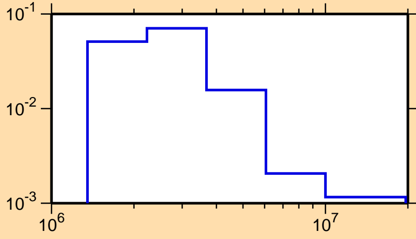
\sigma vs. E for ^{95}\text{Zr}(n,n_4)
