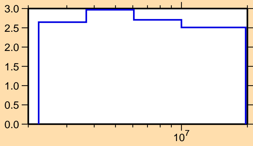
\Delta\sigma/\sigma vs. E for ^{95}\text{Zr}(n,n\text{onel.})
