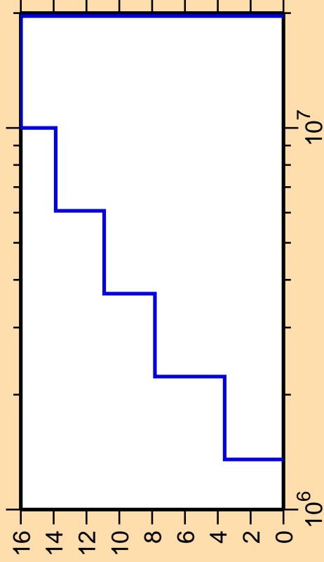
\Delta\sigma/\sigma vs. E for ^{95}\text{Zr}(n,n_4)
