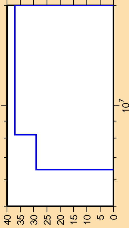
\Delta\sigma/\sigma vs. E for ^{95}\text{Zr}(n,\gamma)
