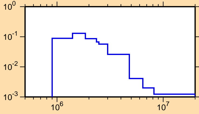
\sigma vs. E for ^{95}\text{Zr}(n,n_1)
