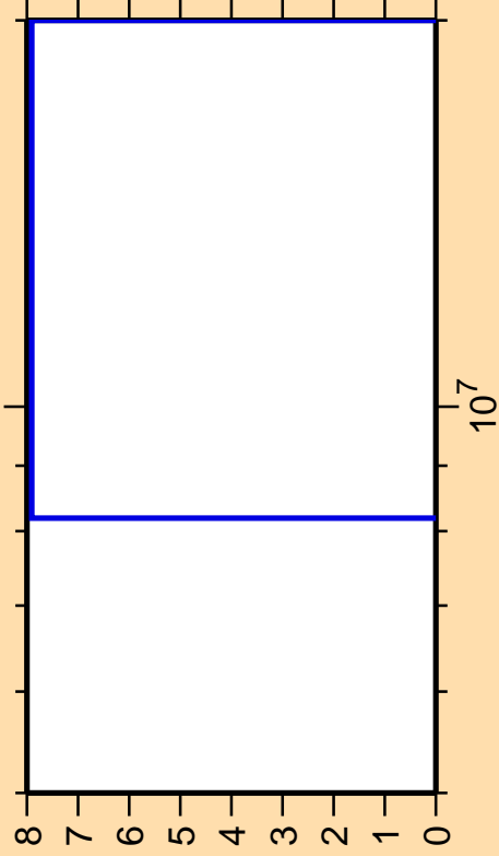
\Delta\sigma/\sigma vs. E for ^{95}\text{Zr}(n,2np)
