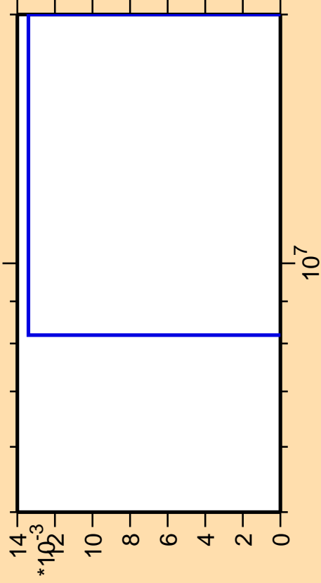
\Delta\sigma/\sigma vs. E for ^{95}\text{Zr}(n,\text{He3})
