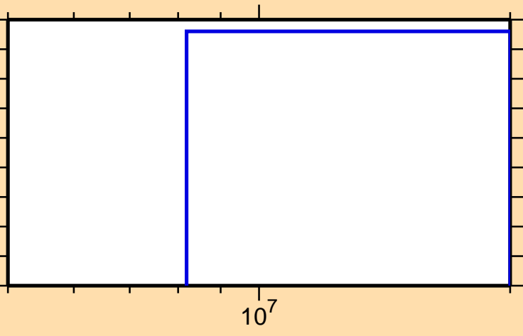
\sigma vs. E for ^{95}\text{Zr}(n,t)
