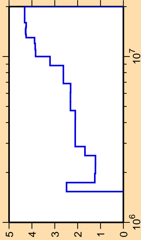
\Delta\sigma/\sigma vs. E for ^{96}\text{Zr}(n,\text{inel.})
