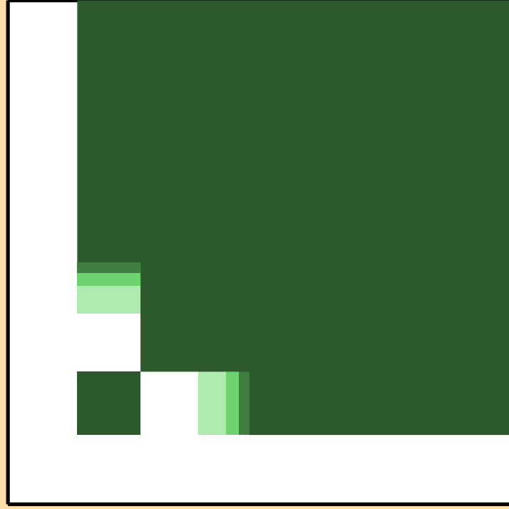
\sigma vs. E for ^{96}\text{Zr}(n,np)
