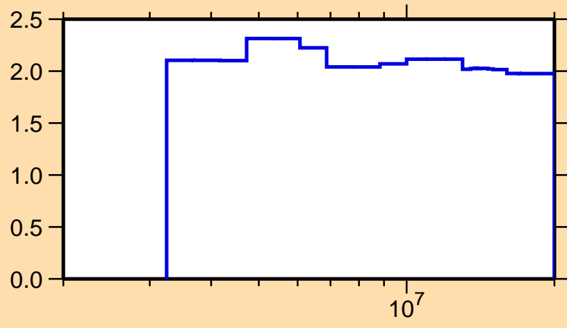
\Delta\sigma/\sigma vs. E for ^{96}\text{Zr}(n,n\text{onel.})
