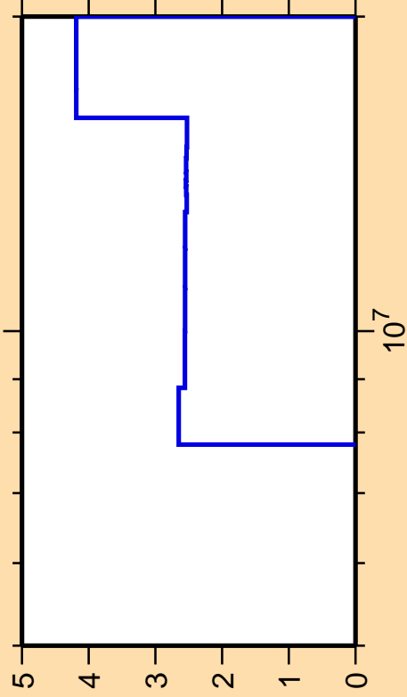
\Delta\sigma/\sigma vs. E for ^{96}\text{Zr}(n,2n)
