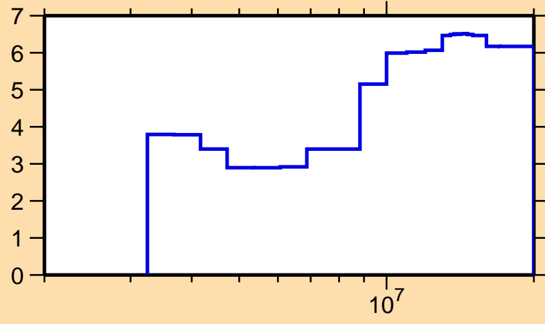
\Delta\sigma/\sigma vs. E for ^{96}\text{Zr}(n,n\text{cont.})
