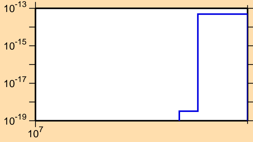
\sigma vs. E for ^{96}\text{Zr}(n,\text{He3})
