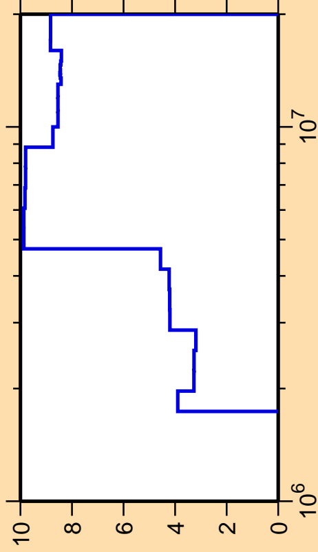
\Delta\sigma/\sigma vs. E for ^{96}\text{Zr}(n,n_3)
