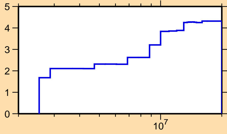
\Delta\sigma/\sigma vs. E for ^{96}\text{Zr}(n,\text{inel.})
