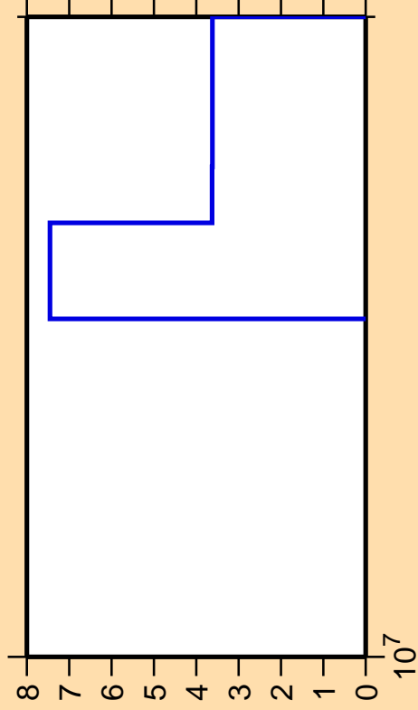
\Delta\sigma/\sigma vs. E for ^{96}\text{Zr}(n,3n)
