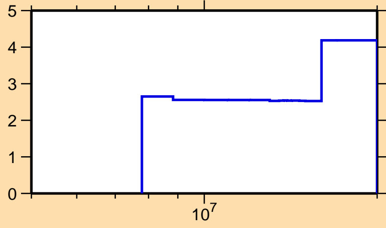
\Delta\sigma/\sigma vs. E for ^{96}\text{Zr}(n,2n)
