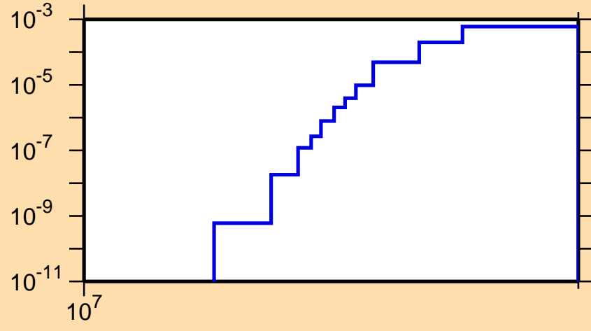
\sigma vs. E for ^{96}\text{Zr}(n,t)
