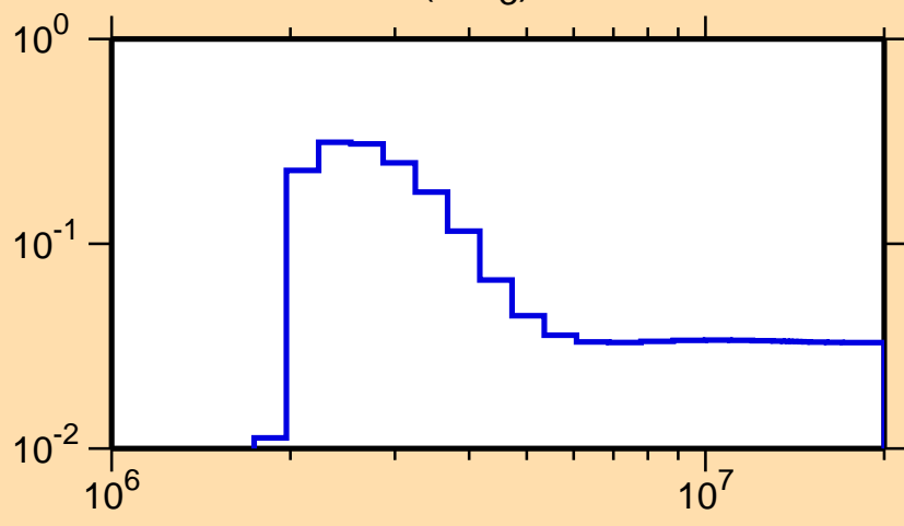
\sigma vs. E for ^{96}\text{Zr}(n,n_3)
