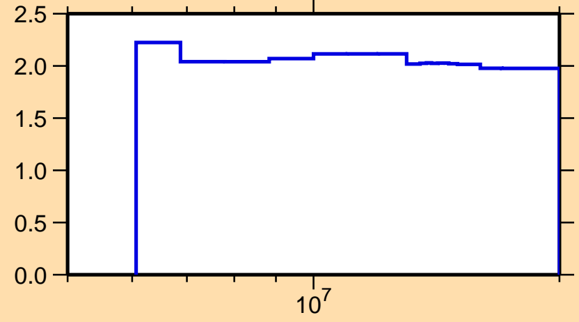
\Delta\sigma/\sigma vs. E for ^{96}\text{Zr}(n,\text{nonel.})
