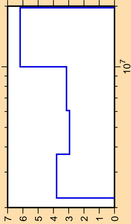
\Delta\sigma/\sigma vs. E for ^{96}\text{Zr}(n,n\text{cont.})
