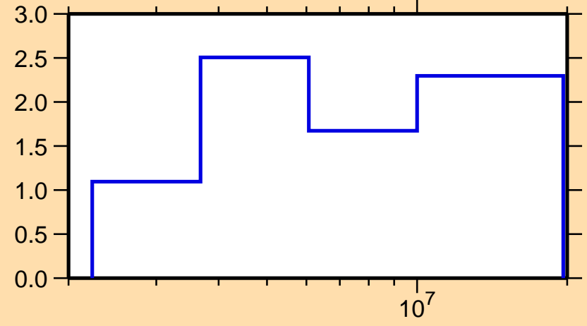
\Delta\sigma/\sigma vs. E for ^{96}\text{Zr}(n,\text{el.})
