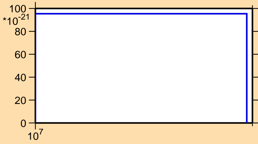
\sigma vs. E for ^{96}\text{Zr}(n,3n\alpha)
