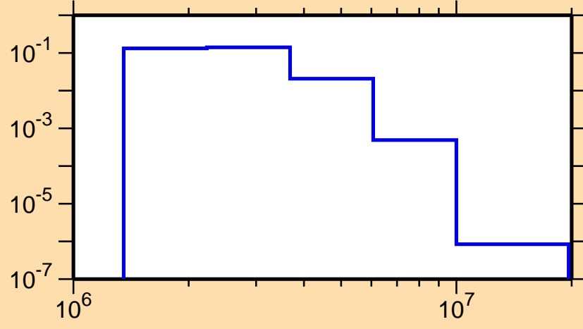
\sigma vs. E for ^{96}\text{Zr}(n,n_1)
