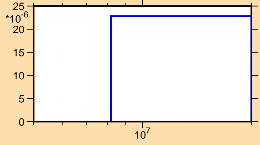
\sigma vs. E for ^{96}\text{Zr}(n,n\alpha)
