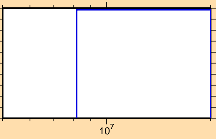
\sigma vs. E for ^{96}\text{Zr}(n,t)
