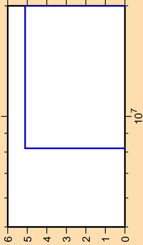
\Delta\sigma/\sigma vs. E for ^{96}\text{Zr}(n,2n\alpha)
