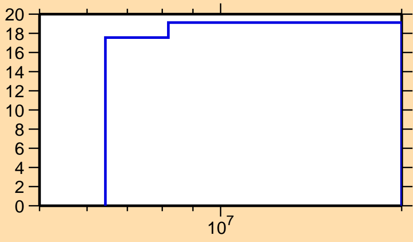
\Delta\sigma/\sigma vs. E for ^{96}\text{Zr}(n,n_1)
