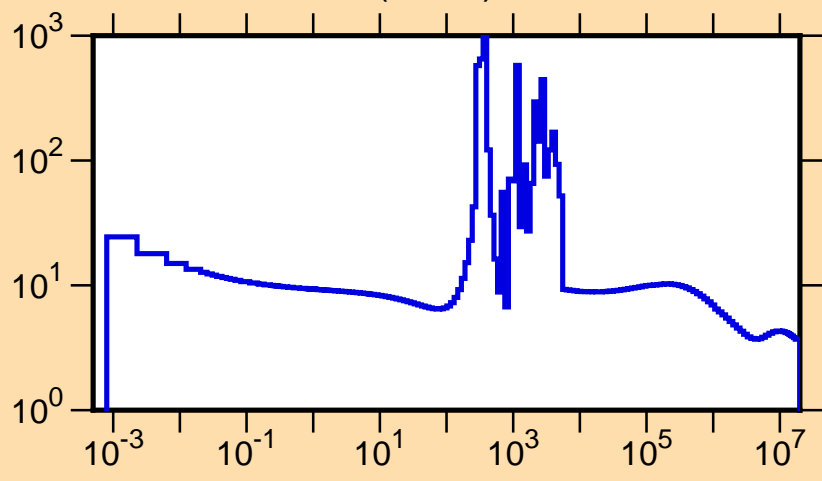
\sigma vs. E for ^{97}\text{Zr}(n,\text{tot.})
