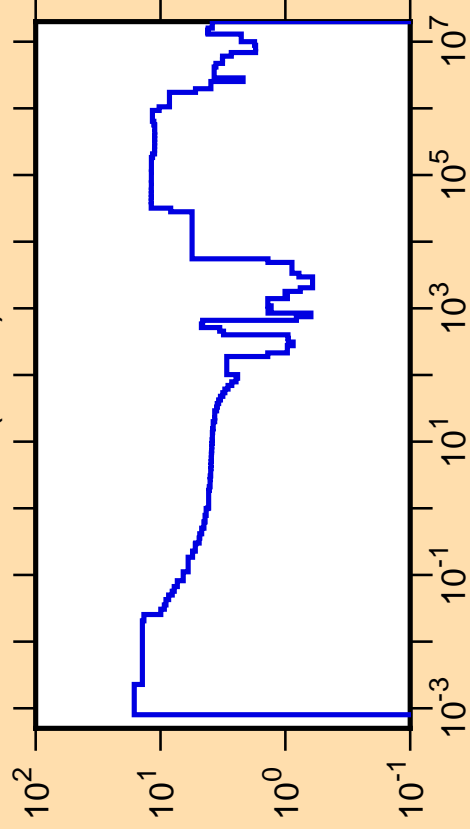
\Delta\sigma/\sigma vs. E for ^{97}\text{Zr}(n,\text{tot.})
