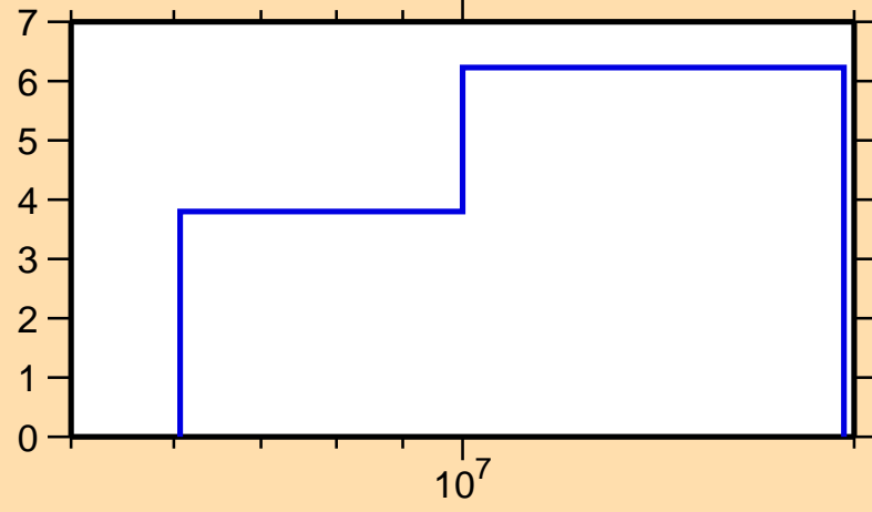
\Delta\sigma/\sigma vs. E for ^{97}\text{Zr}(n,el.)
