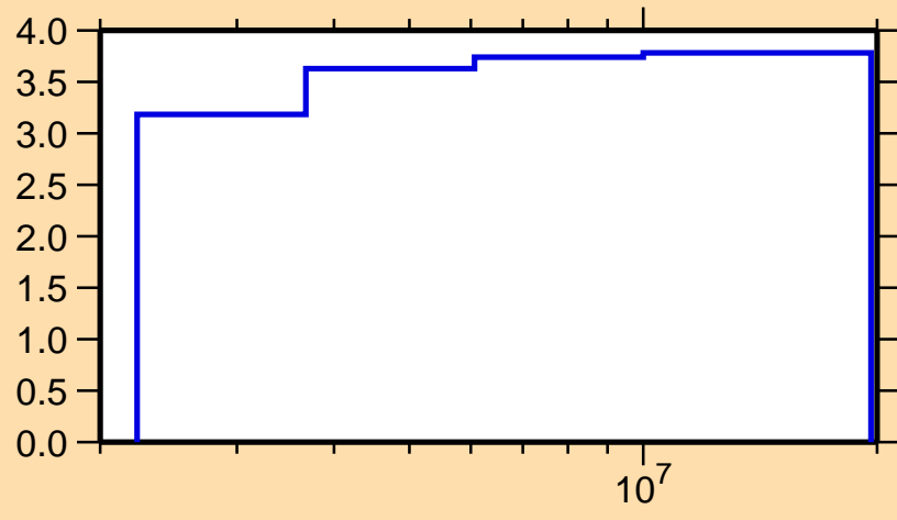
\Delta\sigma/\sigma vs. E for ^{97}\text{Zr}(n,n\text{onel.})
