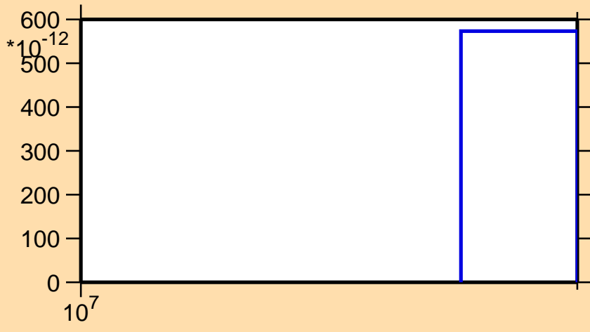
\sigma vs. E for ^{99}\text{Zr}(n,2np)
