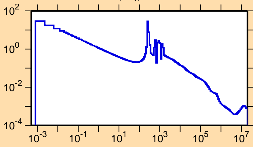
\sigma vs. E for ^{99}\text{Zr}(n,\gamma)
