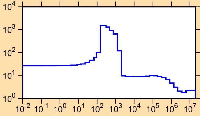
\sigma vs. E for ^{99}\text{Zr}(n,\text{el.})
