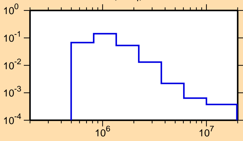
\sigma vs. E for ^{99}\text{Zr}(n,n_4)
