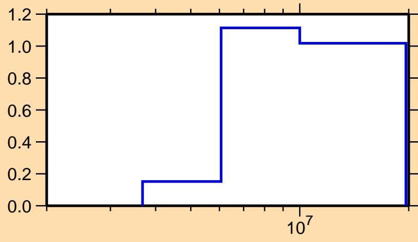
\sigma vs. E for ^{99}\text{Zr}(n,2n)
