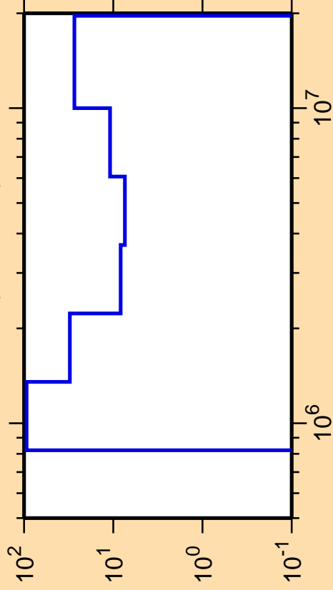
\Delta\sigma/\sigma vs. E for ^{99}\text{Zr}(n,n\text{cont.})
