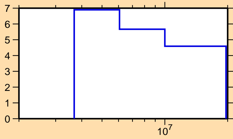
\Delta\sigma/\sigma vs. E for ^{99}\text{Zr}(n,\text{nonel.})
