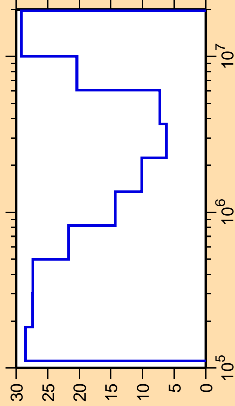
\Delta\sigma/\sigma vs. E for ^{99}\text{Zr}(n,\text{inel.})
