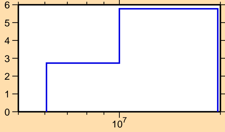
\Delta\sigma/\sigma vs. E for ^{99}\text{Zr}(n,\text{tot.})
