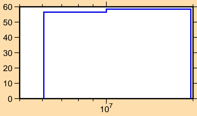
\Delta\sigma/\sigma vs. E for ^{99}\text{Zr}(n,p)
