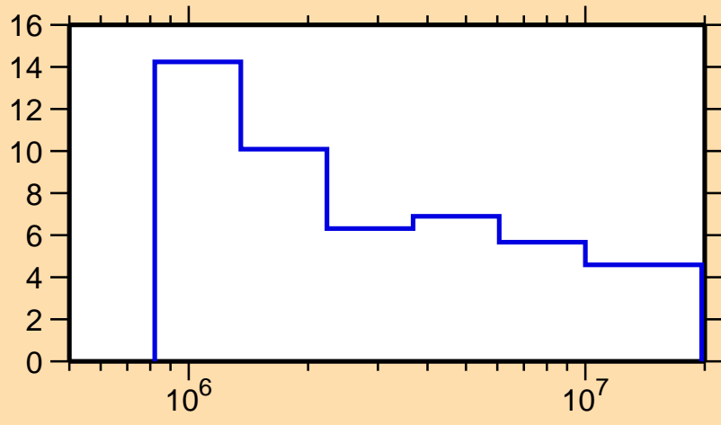
\Delta\sigma/\sigma vs. E for ^{99}\text{Zr}(n,n\text{onel.})
