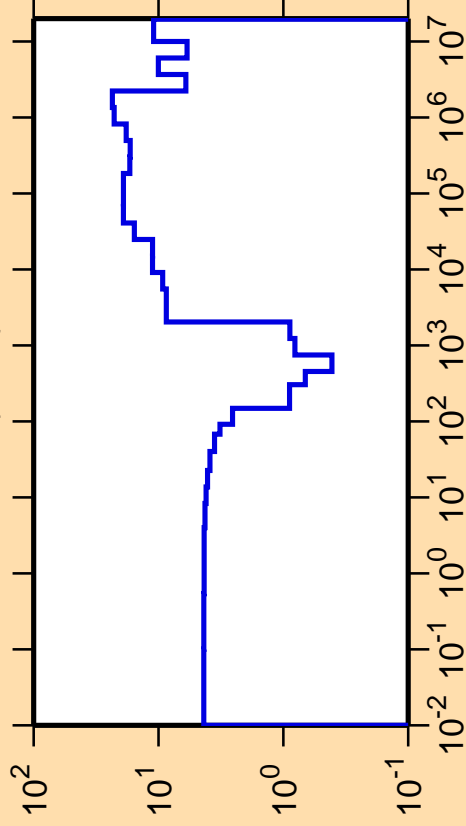
\Delta\sigma/\sigma vs. E for ^{99}\text{Zr}(n,\text{el.})
