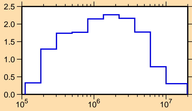
\sigma vs. E for ^{99}\text{Zr}(n,\text{inel.})
