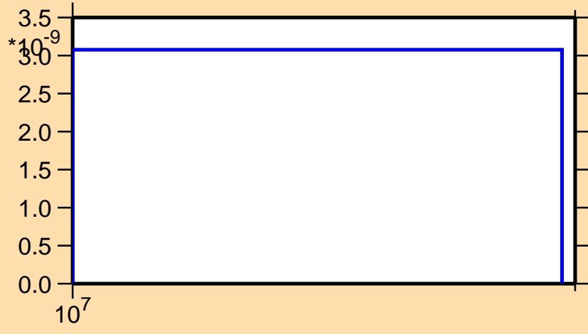
\sigma vs. E for ^{99}\text{Zr}(n,nt)
