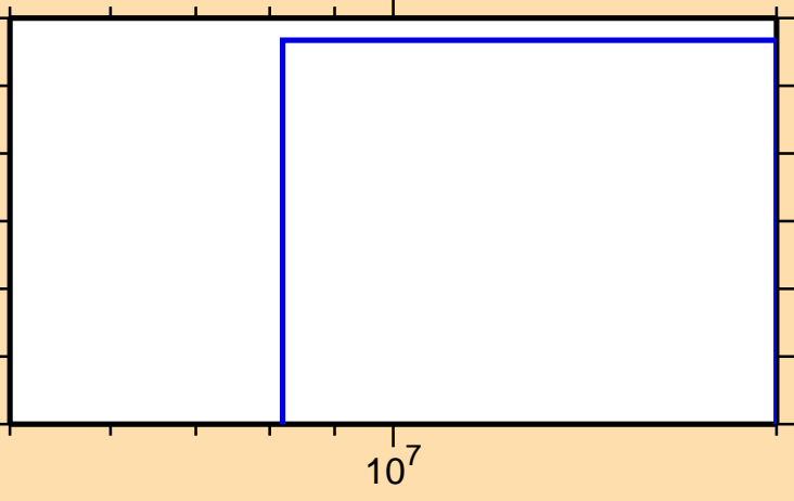
\sigma vs. E for ^{99}\text{Zr}(n,\text{nd})
