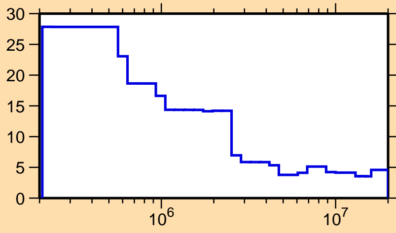
\Delta\sigma/\sigma vs. E for ^{100}\text{Zr}(n,\text{nonel.})
