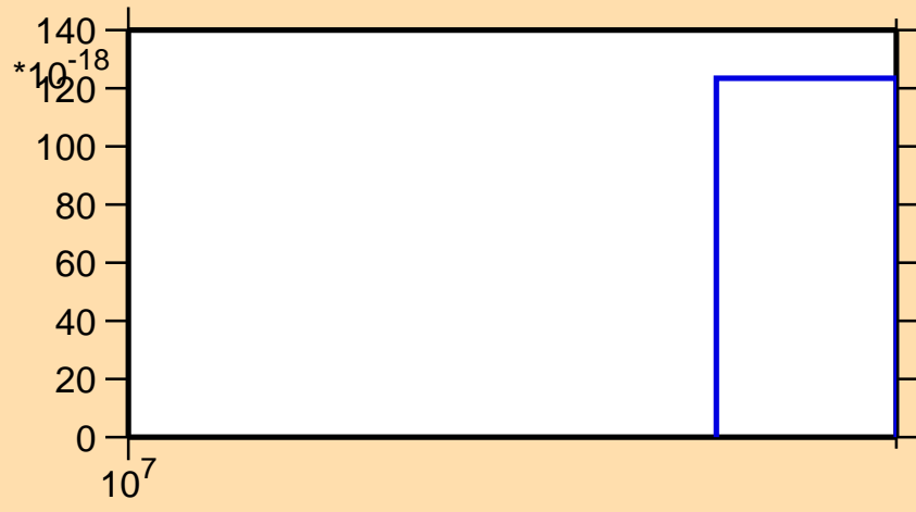
\sigma vs. E for ^{100}\text{Zr}(n,2np)
