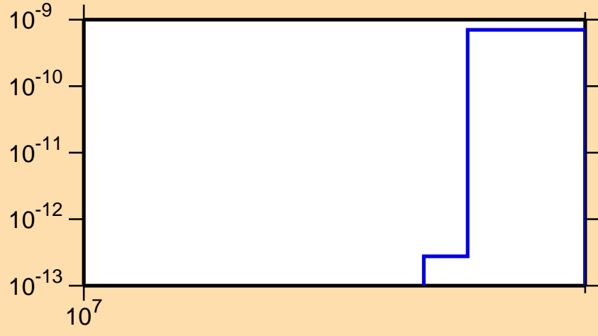
\sigma vs. E for ^{100}\text{Zr}(n,2n\alpha)
