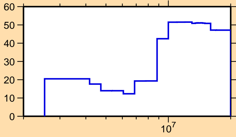
\Delta\sigma/\sigma vs. E for ^{100}\text{Zr}(n,n\text{cont.})
