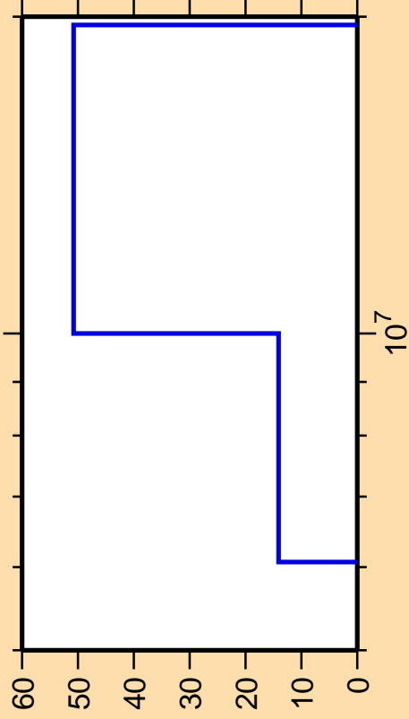
\Delta\sigma/\sigma vs. E for ^{100}\text{Zr}(n,n\text{cont.})
