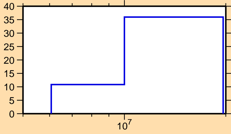
\Delta\sigma/\sigma vs. E for ^{100}\text{Zr}(n,\text{inel.})
