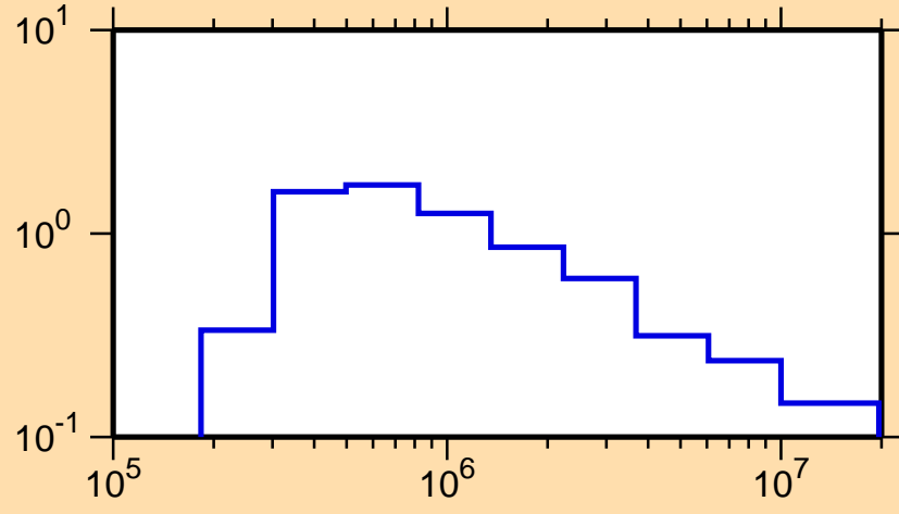
\sigma vs. E for ^{100}\text{Zr}(n,n_1)
