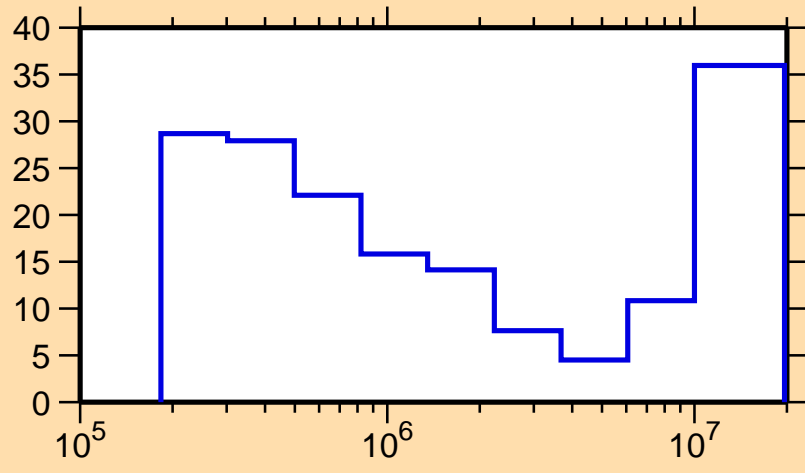
\Delta\sigma/\sigma vs. E for ^{100}\text{Zr}(n,\text{inel.})
