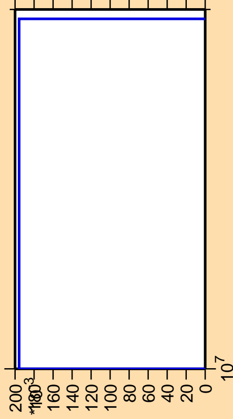
\Delta\sigma/\sigma vs. E for ^{100}\text{Zr}(n,nd)
