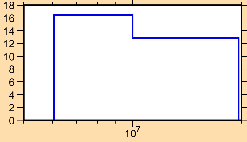
\Delta\sigma/\sigma vs. E for ^{100}\text{Zr}(n,2n)
