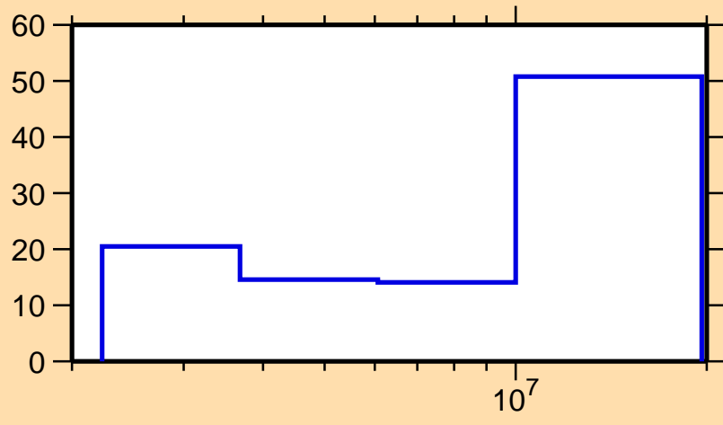
\Delta\sigma/\sigma vs. E for ^{100}\text{Zr}(n,n\text{cont.})
