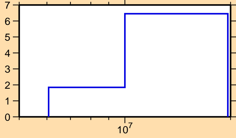
\Delta\sigma/\sigma vs. E for ^{100}\text{Zr}(n,\text{tot.})
