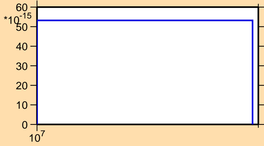
\sigma vs. E for ^{100}\text{Zr}(n,nd)
