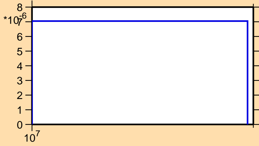
\sigma vs. E for ^{100}\text{Zr}(n,d)
