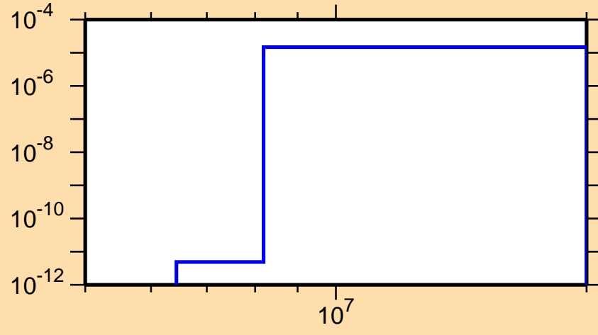
\sigma vs. E for ^{100}\text{Zr}(n,\alpha)
