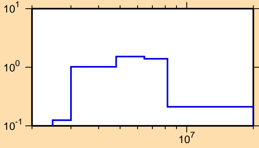
\sigma vs. E for ^{100}\text{Zr}(n,n\text{cont.})
