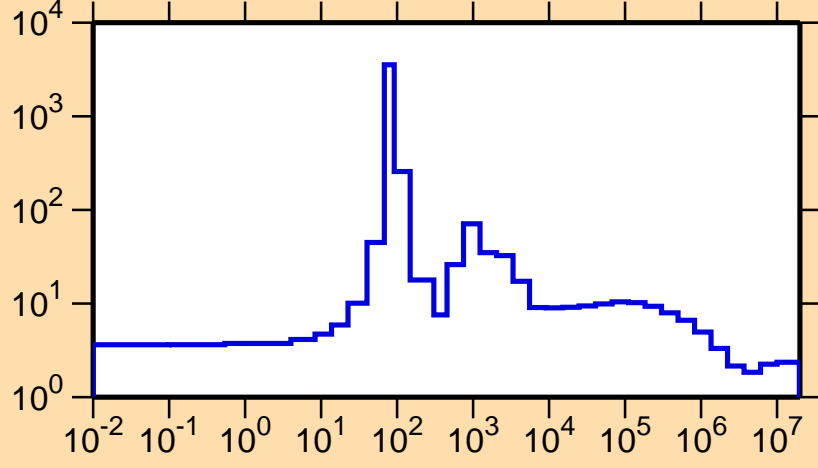
\sigma vs. E for ^{101}\text{Zr}(n,\text{el.})
