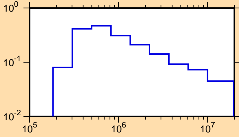
\sigma vs. E for ^{101}\text{Zr}(n,n_2)
