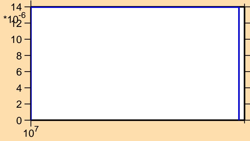
\sigma vs. E for ^{101}\text{Zr}(n,d)
