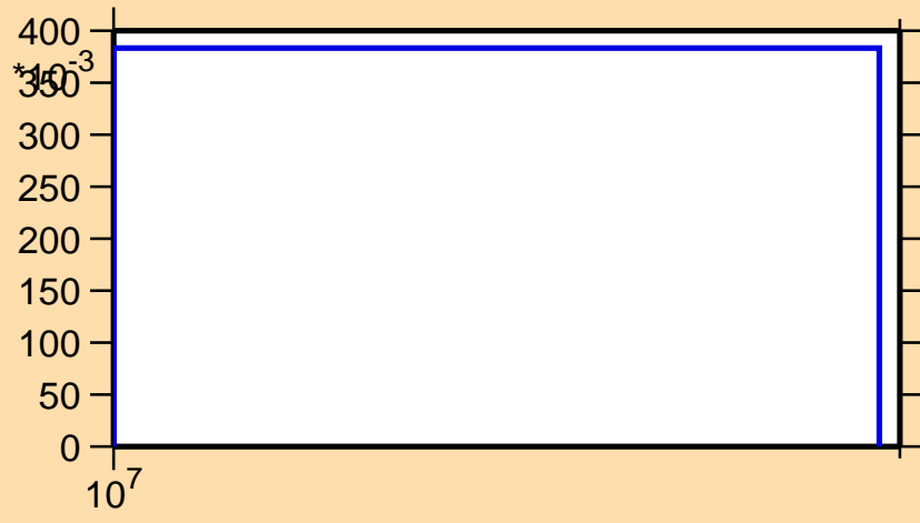
\sigma vs. E for ^{101}\text{Zr}(n,3n)
