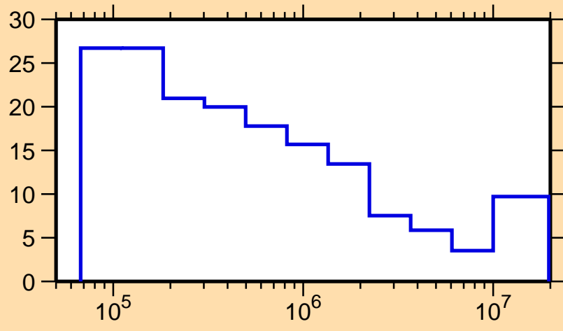
\Delta\sigma/\sigma vs. E for ^{101}\text{Zr}(n,\text{tot.})
