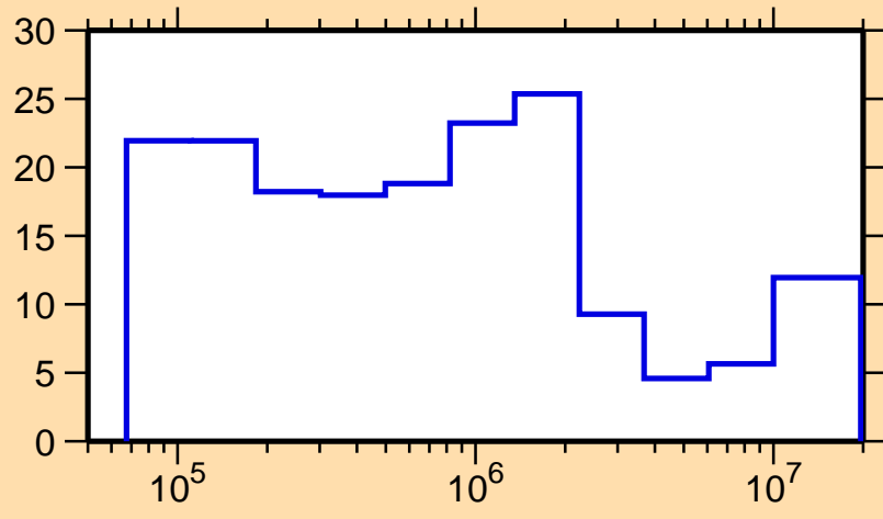
\Delta\sigma/\sigma vs. E for ^{101}\text{Zr}(n,\text{el.})
