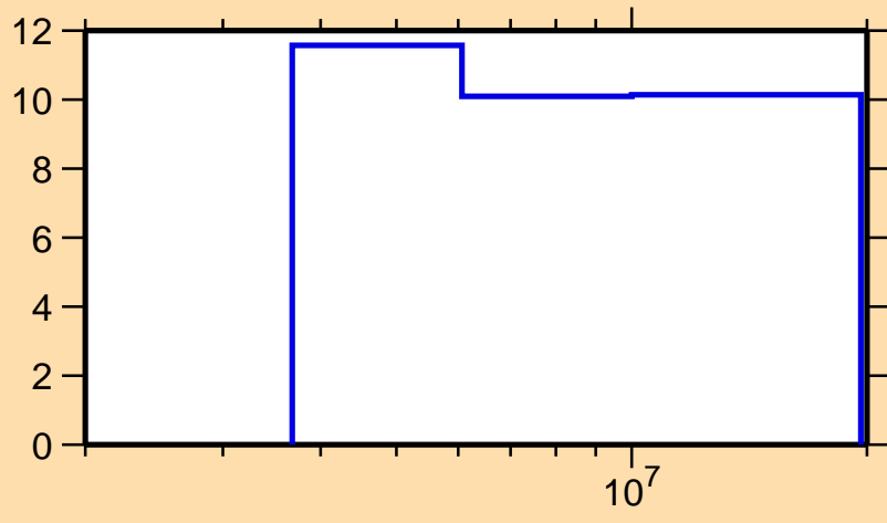
\Delta\sigma/\sigma vs. E for ^{101}\text{Zr}(n,\text{nonel.})
