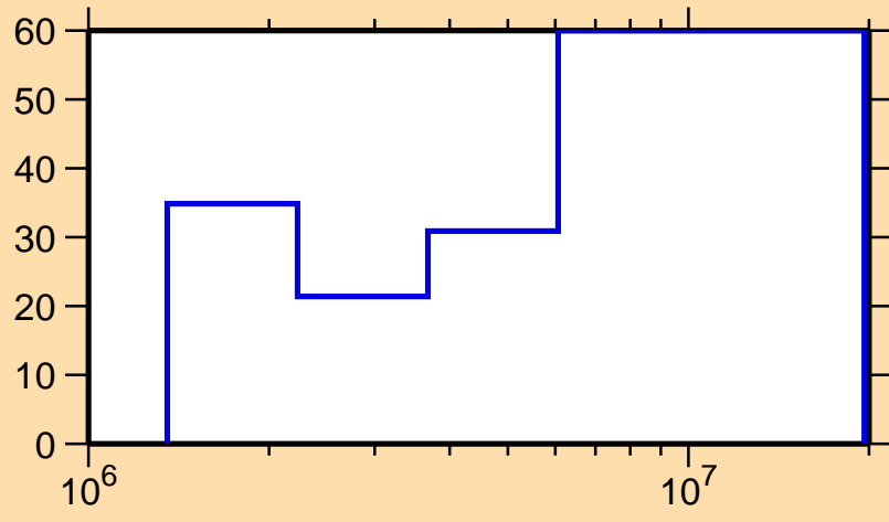
\Delta\sigma/\sigma vs. E for ^{101}\text{Zr}(n,n\text{cont.})
