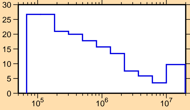
\Delta\sigma/\sigma vs. E for ^{101}\text{Zr}(n,\text{tot.})
