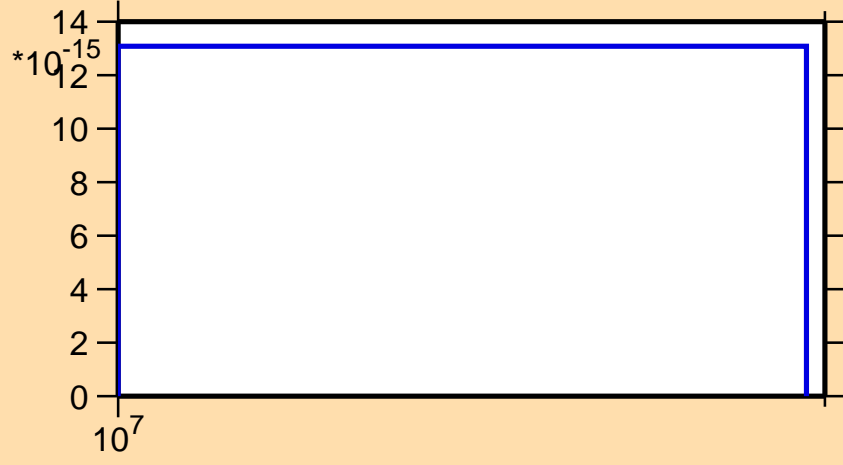
\sigma vs. E for ^{101}\text{Zr}(n,2np)
