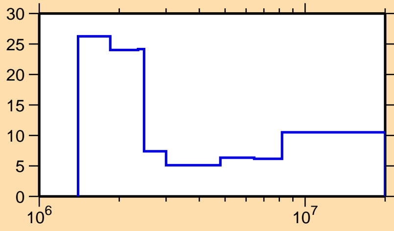
\Delta\sigma/\sigma vs. E for ^{101}\text{Zr}(n, el.)
