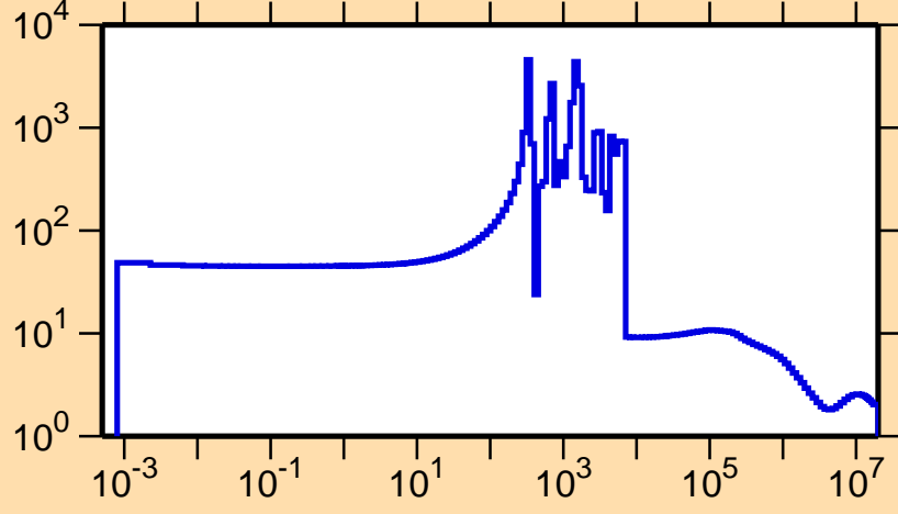
\sigma vs. E for ^{102}\text{Zr}(n,\text{el.})
