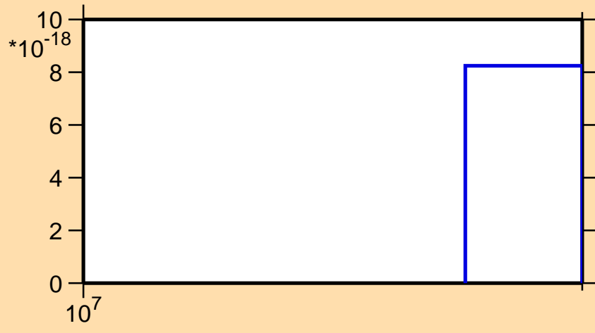
\sigma vs. E for ^{102}\text{Zr}(n,2np)
