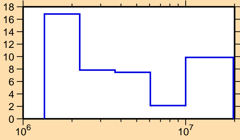
\Delta\sigma/\sigma vs. E for ^{102}\text{Zr}(n,tot.)
