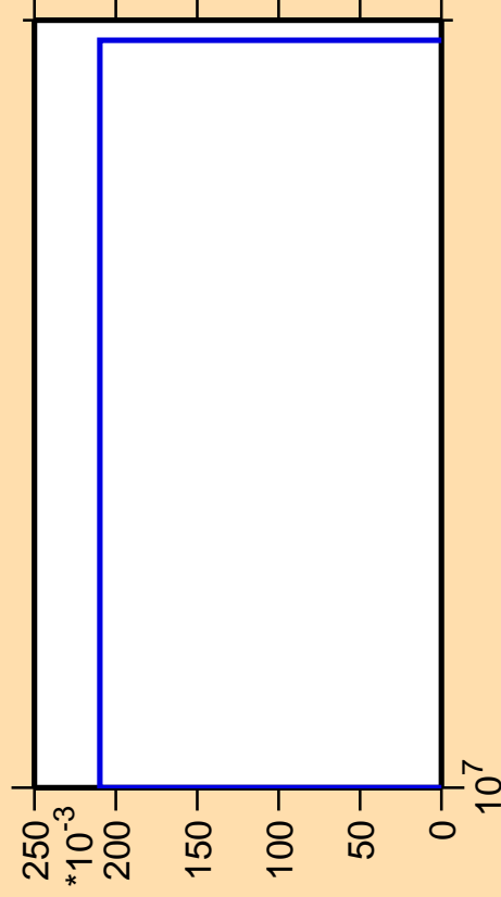
\Delta\sigma/\sigma vs. E for ^{102}\text{Zr}(n,nd)
