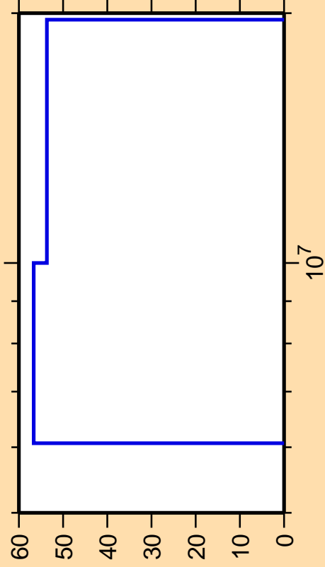
\Delta\sigma/\sigma vs. E for ^{102}\text{Zr}(n,n_1)
