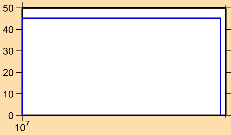
\Delta\sigma/\sigma vs. E for ^{102}\text{Zr}(n,ncont.)
