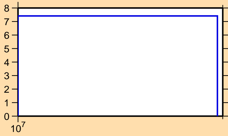
\Delta\sigma/\sigma vs. E for ^{102}\text{Zr}(n,\text{nonel.})
