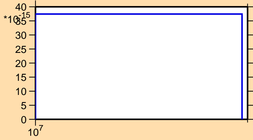
\sigma vs. E for ^{102}\text{Zr}(n,nd)
